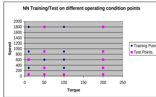
Figure 4. Operating points used for generating, training and testing data. Torque is measured in the unit of nm, and speed is in rpm.
