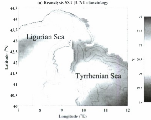
Figure 2. Climatological mean SST, and bathymetry, for the Ligurian and Tyrrhenian Sea for June. SST is got from the GOS CNR reanalysis products. Bathymetry is contoured at 2000m, 500m, 100m (solid) and 1000m, 200m, 50m (dash).
