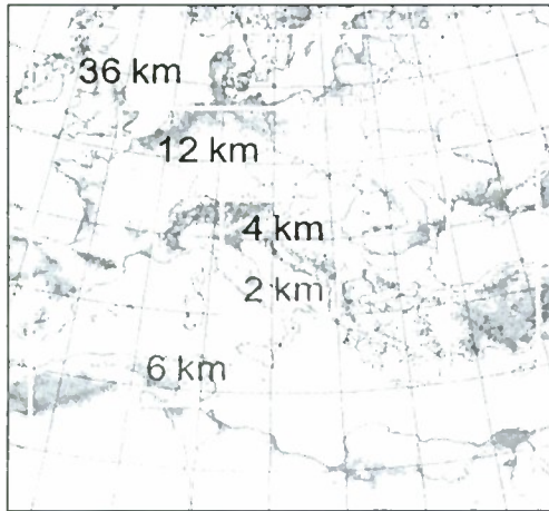
Fig. 1: Atmospheric and ocean grid setup for the Adriatic Sea. The resolution for the atmospheric nests (black) and the ocean nests (purple) are indicated.
