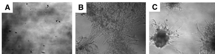
Fig. 2 – Bovine serum exosome mediated growth of stellate colonies of breast cancer cells in Matrigel. Liquid Matrigel (100 \mu\text{l}/\text{well} ) was allowed to solidify at 37^\circ\text{C} in 96-well micro titer plate. The carcinoma cells were then added on the Matrigel (500 cells/well) in the presence of serum free medium (panel A), exosome-free medium (panel B) and exosome enriched medium (panel C). The cells were then incubated in a humidified \text{CO}_2 incubator for 14 days and then photographed.
