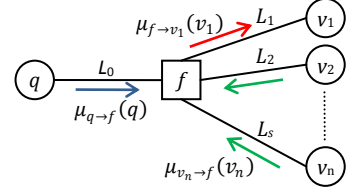
Figure 5: The most time consuming part of the belief propagation algorithm in our case: to send a message, \mu_{f \rightarrow v_i}(v_i) in red, from a projection factor node f (in level 3 of Figure 2) to a voxel variable node v_i (in level 2). This factor node has already received messages from the pixel occupancy q (in level 4), \mu_{q \rightarrow f}(q) in blue, and from the voxels, \mu_{v_j \rightarrow f}(v_j) in green. A general implementation computes this message in O(2^n) complexity ( n is the number of voxels in the line of sight of the pixel), whereas our implementation has complexity O(n^d) .
