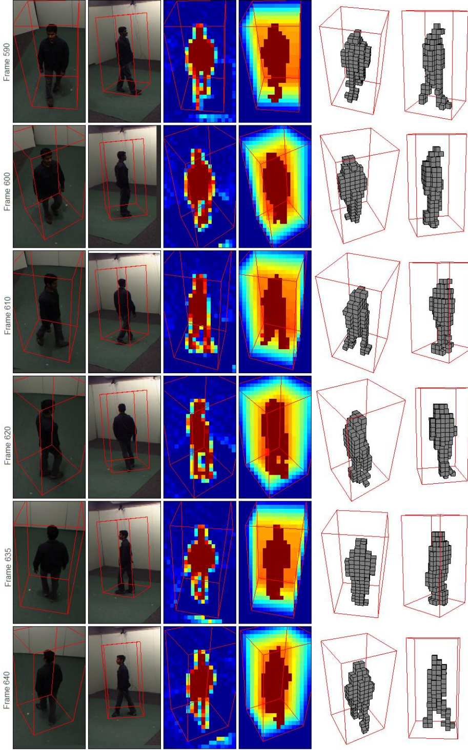
Figure 7: Reconstructions for six frames in the testing dataset when the registration parameters are known. The best and worst three reconstructions (according to reconstruction error) are shown in the first and last three rows, respectively. The bounding boxes were included in all images (in red).
