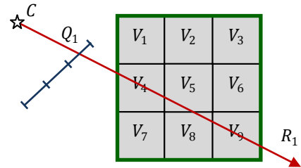
Figure 3: 2D analog of the projection process. A ray R_1 , originating at the camera center C , passes through its corresponding pixel Q_1 in the image plane (in blue) and intersects the voxels in its line of sight ( V_4, V_5, V_8 and V_9 ) inside the 2D bounding box (in green). The relationship among these particular variables is depicted in the factor graph of Figure 2.
