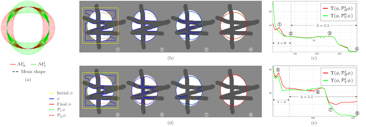
Fig. 3. (a) Mode of variation for the two ellipses models ($\mathcal{M}_V^1$ in green and $\mathcal{M}_H^1$ in red), the mean shape of both models is the same and is plotted in black dash line. (b) Results for the experiments with $\mathcal{M}_H^1$ and $\mathcal{M}_V^0$ (only mean shape). Some steps in the segmentation (see text) (c) Evolution of the shape dissimilarity measure for the experiments with $\mathcal{M}_H^1$ and $\mathcal{M}_V^0$. (d) Results for experiments with $\mathcal{M}_H^1$ and $\mathcal{M}_V^1$ (complete model). (e) Evolution of the shape dissimilarity measure for the experiments with $\mathcal{M}_H^1$ and $\mathcal{M}_V^1$. (This figure is in colors.)
