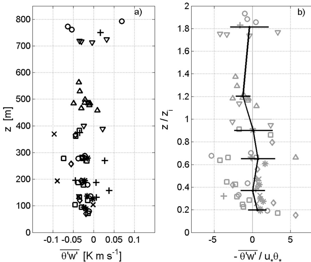
FIG. 6. Vertical profiles of the (a) covariances of potential temperature and vertical velocity, and (b) dimensionless covariances with height normalized by the mixed layer depth. Symbols are the same as in Fig. 4.
