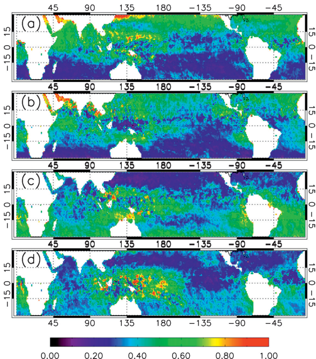
FIG. 1. Fraction of clear-sky observations for 1^\circ \times 1^\circ boxes that have detectable thin cirrus optical depths larger than 0.02 for boreal (a) spring, (b) summer, (c) autumn, and (d) winter. The definition of season is determined by conventional boreal season such that spring months are March, April, and May; summer months are June, July, and August; autumn months are September, October, and November; and winter months are December, January, and February.
