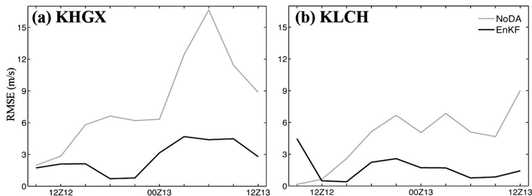
FIG. 6. The RMSE of the radial velocity of the EnKF analysis vs the NoDA experiment verified against the 10% independent radial velocity SOs from (a) KHGX and (b) KLCH.
