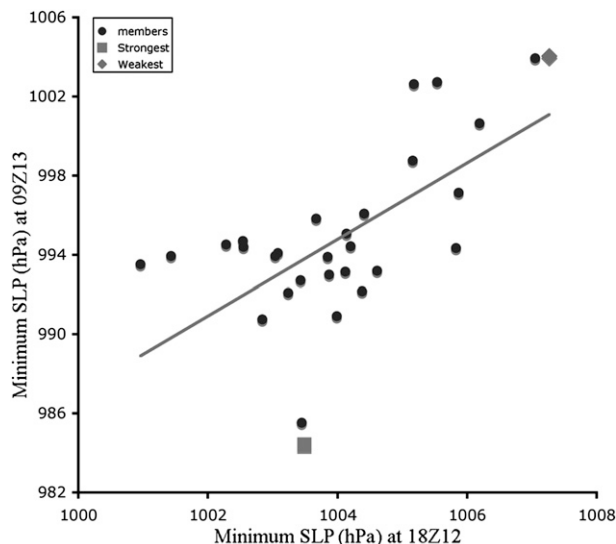
FIG. 13. The scatterplot of the forecasted minimum SLP at 1800 UTC 12 Sep ( x axis; 0 h) and 0900 UTC 13 Sep 2007 ( y axis; 15 h) in different ensemble members with the weakest and strongest members at 0900 UTC 13 Sep highlighted.
