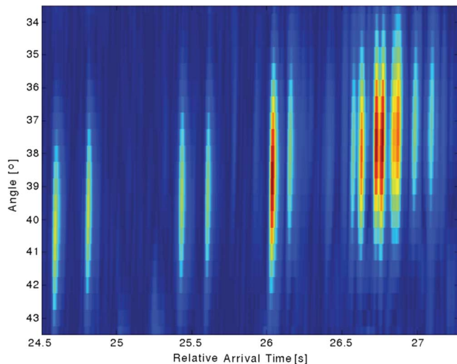
Fig. 12. Beamformed reception showing “ray-like” arrivals with relative intensities as measured on the bottom-mounted horizontal hydrophone array indicated by the letter “R” in Fig. 1. The suspended source was at station T250 and a depth of 800 m. Only one 27.28-s M-sequence was processed for this figure.
