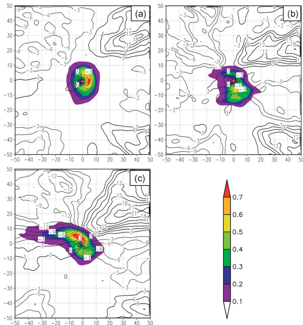
FIG. 6. Composites of the initial SVs (colors) and the radial wind (contours; \text{m s}^{-1} ) at 500 hPa at the initial time for the (a) A, (b) B, and (c) C groups. The TC symbols indicate the composited TC center.
