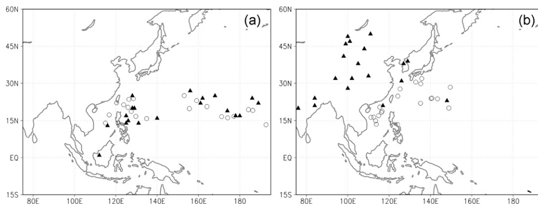
FIG. 4. The locations of initial SV maximum (▲) and the TC center (○) at the initial time for each (a) NI and (b) RI case.
