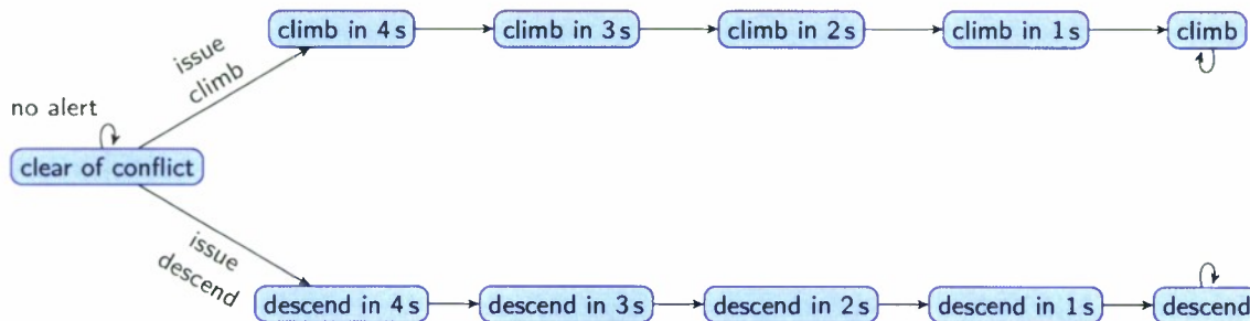
Figure A-1. The variable s_{RA} tracks which RA has been issued and the delay.
