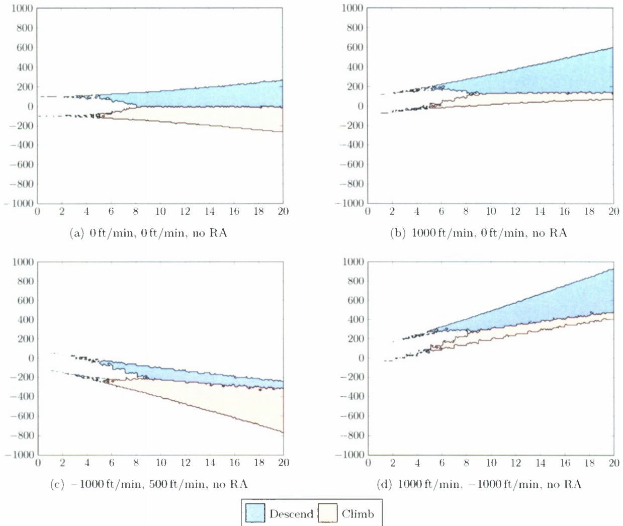
Figure 13. Collision avoidance policy generated by the conservative strategy. The caption of each subfigure indicates the cross section (\dot{h}_1, \dot{h}_2, s_{RA}) for which the policy is evaluated. The horizontal axis represents \tau in seconds, and the vertical axis represents h in feet.
