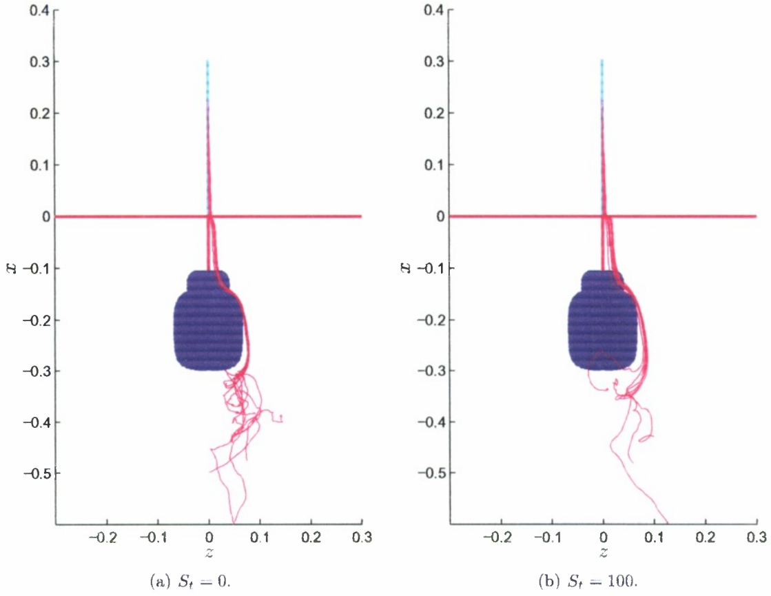
Figure 6: Effect of Stokes number on particle trajectories.
