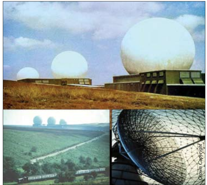
Figure 2. The Original Fylingdales Early Warning Radar.
