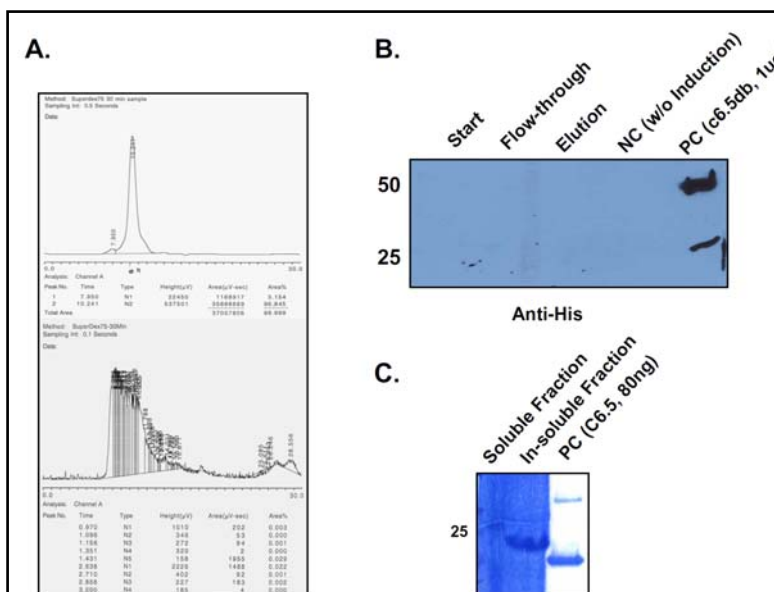
Figure 1. Purification of C6.5-protamine fusion proteins. Purification of C6.5-protamine fusion proteins was determined by HPLC (A. Up panel: C6.5; Low panel: C6.5-protamine) and Western blot analyses (B). (C) The levels of C6.5-protamine fusion protein were also examined by Western blot analysis in protein samples extracted from soluble and insoluble cell fractions. Recombinant C6.5 protein was loaded as positive control (PC).
