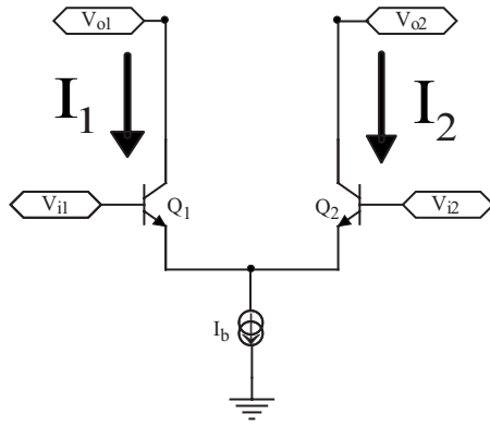
FIG. 1. The differential pair is used as the basic building block in the bistable elements. It consists of two transistors ( Q_1 and Q_2 ) and a current source.
