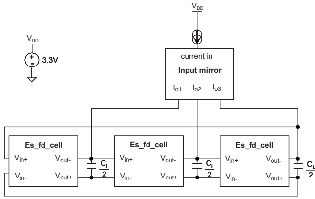
FIG. 4. Top-level schematic of a circuit realization of a coupled electric-field system with three units coupled unidirectionally.
