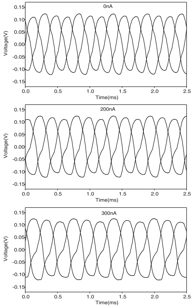
FIG. 14. Time series from the experimental system. Each graph shows the three waveforms from the three oscillators used in the coupled network. The first graph (top) shows the oscillations with zero applied current. The second graph is for applied current I_{\text{sig}} = 200 nA. The third graph (bottom) is for the applied current I_{\text{sig}} = 300 nA.
