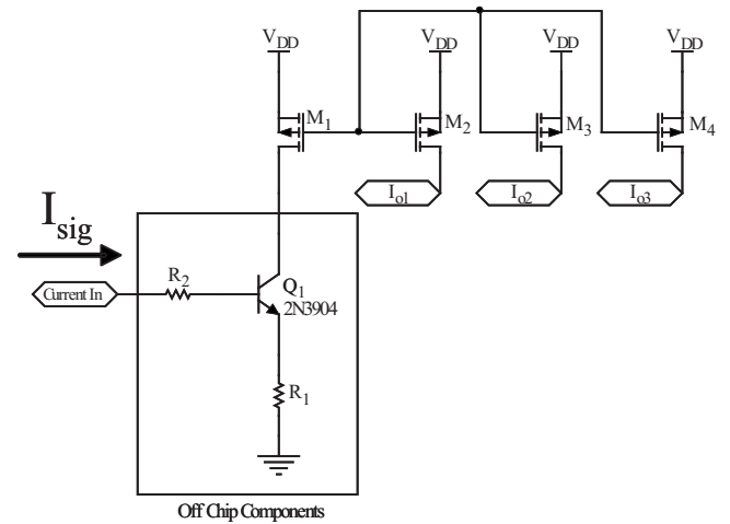
FIG. 3. The input current mirror provides the same current to each of the bistable elements of the coupled system shown in Fig. 4.
