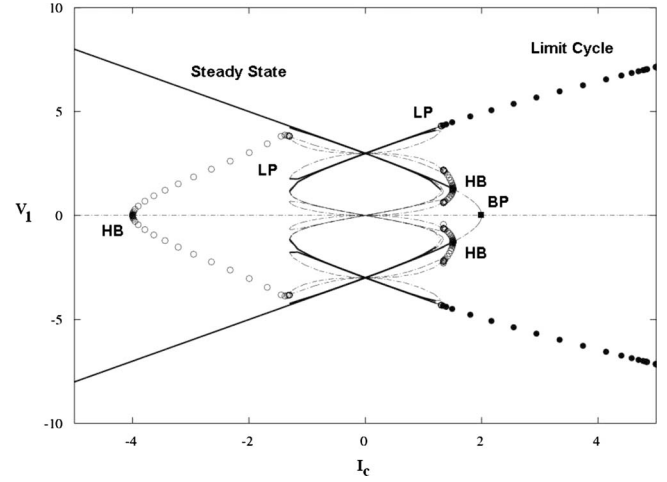
FIG. 5. Bifurcation diagram for a coupled ( N=3 ) electric-field sensor microcircuit showing the system's voltage output in response to changes in coupling parameter I_c . The filled-in circles represent globally, asymptotically, stable limit-cycle oscillations created at the onset, LP, of a heteroclinic bifurcation. The solid lines depict the local branches of stable steady-state solutions. The empty circles correspond to unstable branches of periodic oscillations that emerge via Hopf bifurcations. The parameters are C_L=1 , g=1 , c=1 , I_s=2 and I_c=1 .
