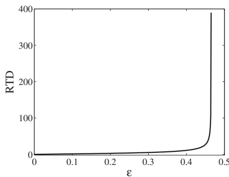
FIG. 9. RTD measures as a function of input signal strength \varepsilon , for a coupled ( N=3 ) electric-field sensor system, obtained from numerical simulations of model equation (3). The sensitivity of the coupled sensor device is proportional to the slope of the RTD curve. Notice that the slope is particularly large near \varepsilon=0.45 , which is near the bifurcation point that leads to oscillatory behavior in the device. The parameters as in Fig. 5.
