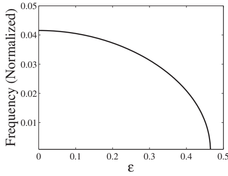
FIG. 8. Frequency response to the input signal \varepsilon for a coupled ( N=3 ) electric-field sensor system, obtained from numerical simulations of model equation (3). The frequency scales by the universal power- \frac{1}{2} law, which is typical for this type of bifurcation scenario. The parameters as in Fig. 5.
