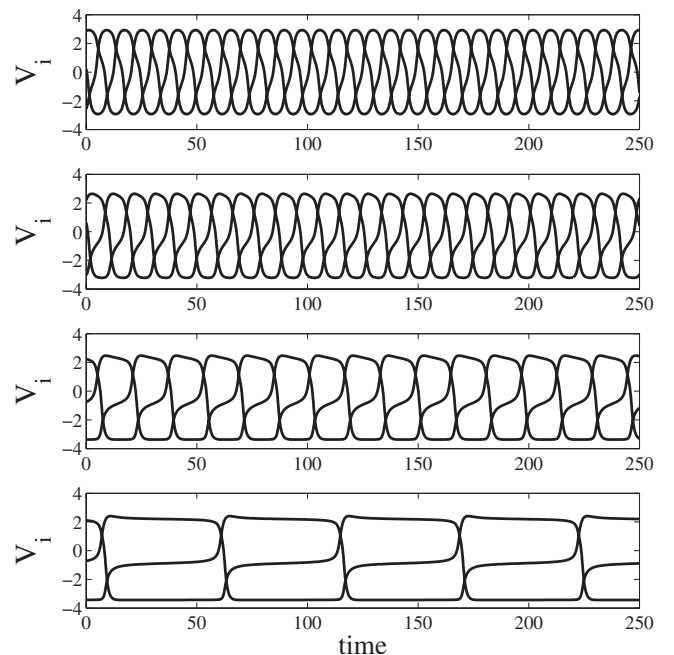
FIG. 7. Time series of oscillatory behavior in a coupled ( N=3 ) electric-field system. As \varepsilon=[0, 0.25, 0.4, 0.46] increases from the top panel to the bottom one, the frequency of the oscillations decreases correspondingly. The parameters as in Fig. 5.
