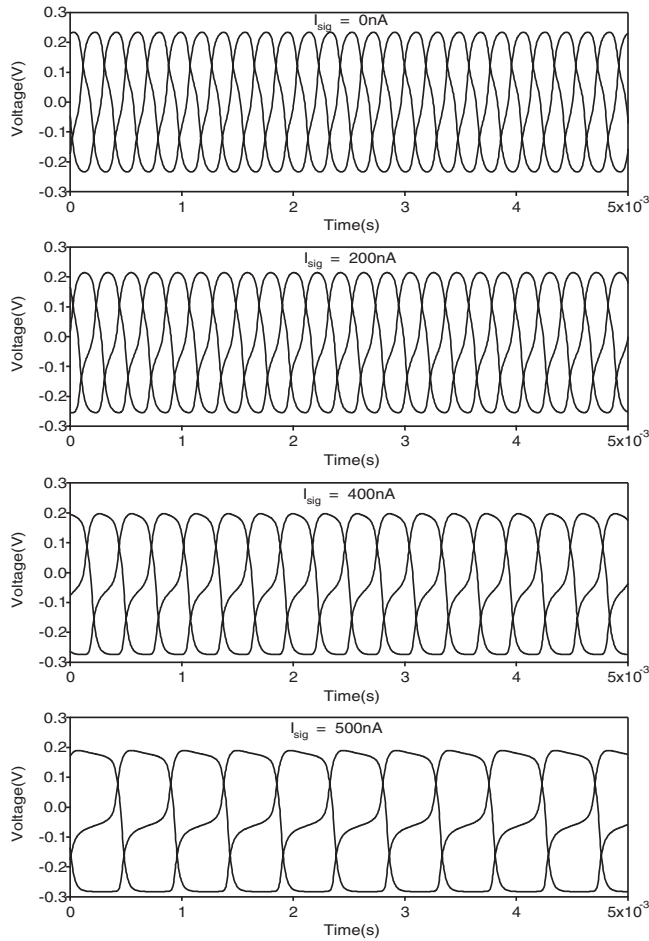
FIG. 11. Waveforms of the differential output from all three coupled elements, from a coupled electric-field sensor device, are plotted for different values of input dc I_{\text{sig}} . The outputs are characteristically out of phase by 2\pi/N(N=3) degrees, so that collectively they form a traveling wave pattern. From top to bottom, I_{\text{sig}} is set to 0, 200, 400, and 500 nA, respectively.
