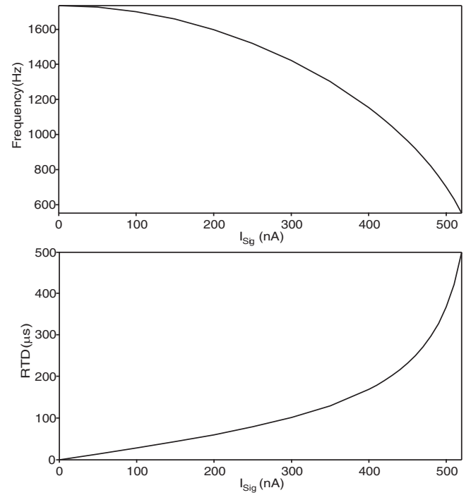
FIG. 12. Frequency and RTD responses of the experimental coupled electric-field sensor system subject to an injected current I_{\text{sig}} . The scaling factor (gain) \beta of the injected current is determined to be approximately 150. Observe the similarity between these two experimental responses and the numerical responses of model equation (3) shown previously in Figs. 8 and 9, respectively.
