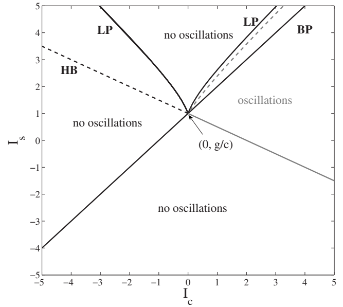
FIG. 6. Two-parameter bifurcation diagram for a coupled ( N=3 ) electric-field system in parameter space (I_s, I_c) . The diagram confirms the existence of an open region where limit-cycle oscillations are globally, asymptotically, stable. The diagram, as well as the stability properties of the solutions found in each region, was determined numerically using continuation software (Ref. 7). The dashed lines represent when the Hopf bifurcation becomes unstable. The parameters as in Fig. 5.
