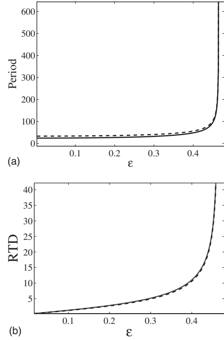
FIG. 10. Comparison of analytical approximations with numerical simulations for (top) period T and (bottom) RTD responses for a coupled electric-field sensor. The solid line indicates analytical approximations obtained through Eqs. (15) and (16), respectively. The dashed lines correspond to numerical results from simulations of hardware dynamics (3).
