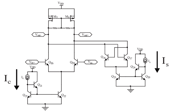
FIG. 2. A single (bistable) element is constructed out of differential pairs. Each element contains a cross coupled pair, input signal circuitry, and coupling components.
