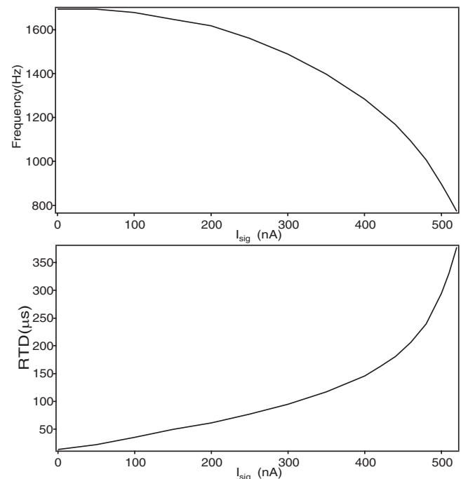
FIG. 13. Frequency and RTD responses of hardware simulations, via SPICE, of a coupled electric-field sensor. Observe the similarity between these two hardware-simulated responses of the design and the numerical responses of model equation (3) shown previously in Figs. 8 and 9, respectively.
