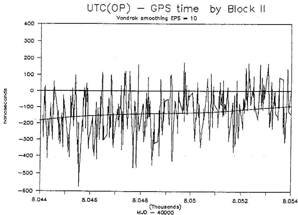
Figure 2. Values of UTC(OP)-GPS time by Block II satellites smoothed over a periode of 10 days.
