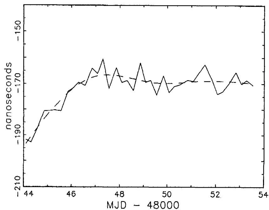
Figure 3. Common-views between Paris Observatory and US Naval Observatory (distance of about 6000km) over a periode of 10 days. Dashed lines represent smoothing.
