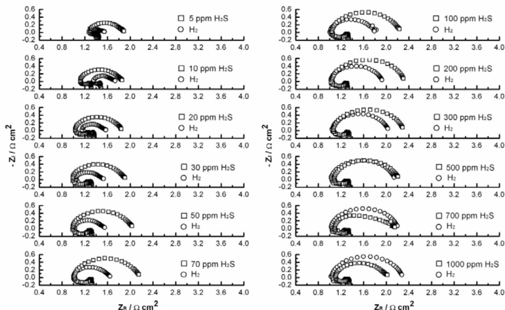
Figure 16. Impedance curves responses of Ni/GDC anodes as a function of H_2S concentration, measured at open circuit condition after polarized at 200 \text{ mA cm}^{-2} for 2 h and 800^\circ\text{C} .
