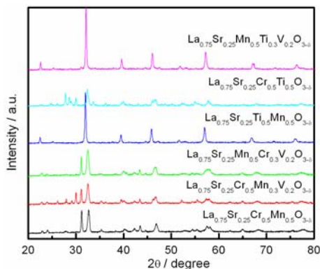
Figure 13. the XRD patterns of oxide powders after baking in 10%H 2 /N 2 at 1100°C for 10 hrs. The powder was pre-calcined at 800°C for 5 hrs
