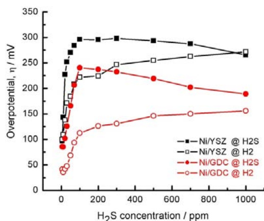
Figure 24. Overpotential of Ni/GDC and Ni/YSZ anodes as a function of H 2 S concentration measured after polarized at 200 mA cm -2 for 2 h and 800 °C.
