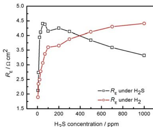
Figure 19. Plots of the anode interfacial resistance of Ni/YSZ anodes as a function of \text{H}_2\text{S} concentration, measured at open circuit condition after polarized at 200 \text{ mA cm}^{-2} for 2 h and 800^\circ\text{C} .
