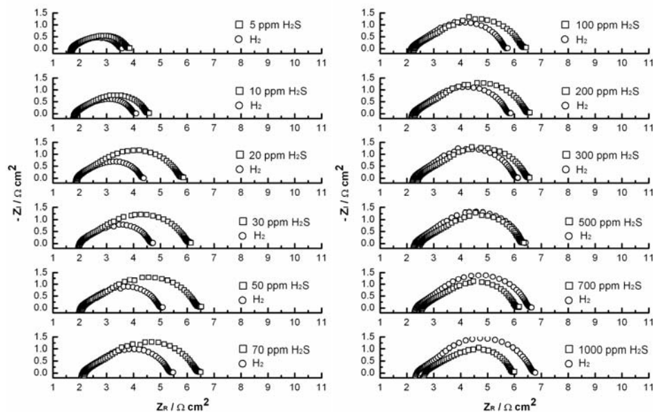
Figure 18. Impedance curves responses of Ni/YSZ anode as a function of \text{H}_2\text{S} concentration, measured at open circuit condition after polarized at 200 \text{ mA cm}^{-2} for 2 h and 800^\circ\text{C} .
