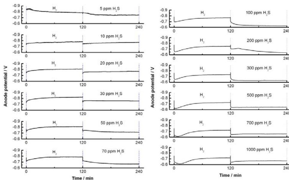
Figure 21. Polarization responses of Ni/GDC anodes as a function of H 2 S concentration measured under anodic current passage at 200 mA cm -2 for 2h and 800°C.
