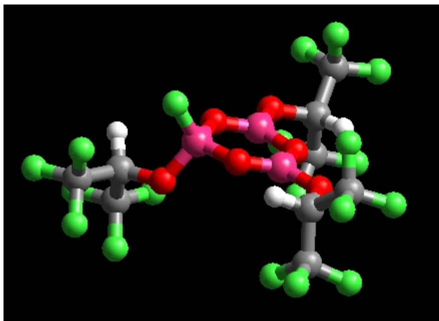
Fig 25. tris(hexafluoroisopropyl)anhydride). Pink= Boron, Red=Oxygen, Grey=Carbon, White=Hydrogen, Green=Fluorine Atoms.
