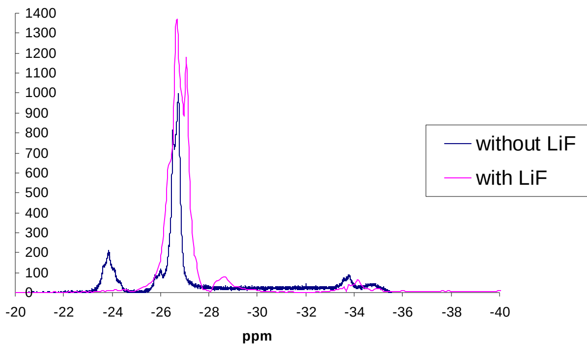
Fig. 9. ^{19}\text{F} NMR data of 0.1M difluorophenyl boroxine in propylene carbonate, with and without LiF.
