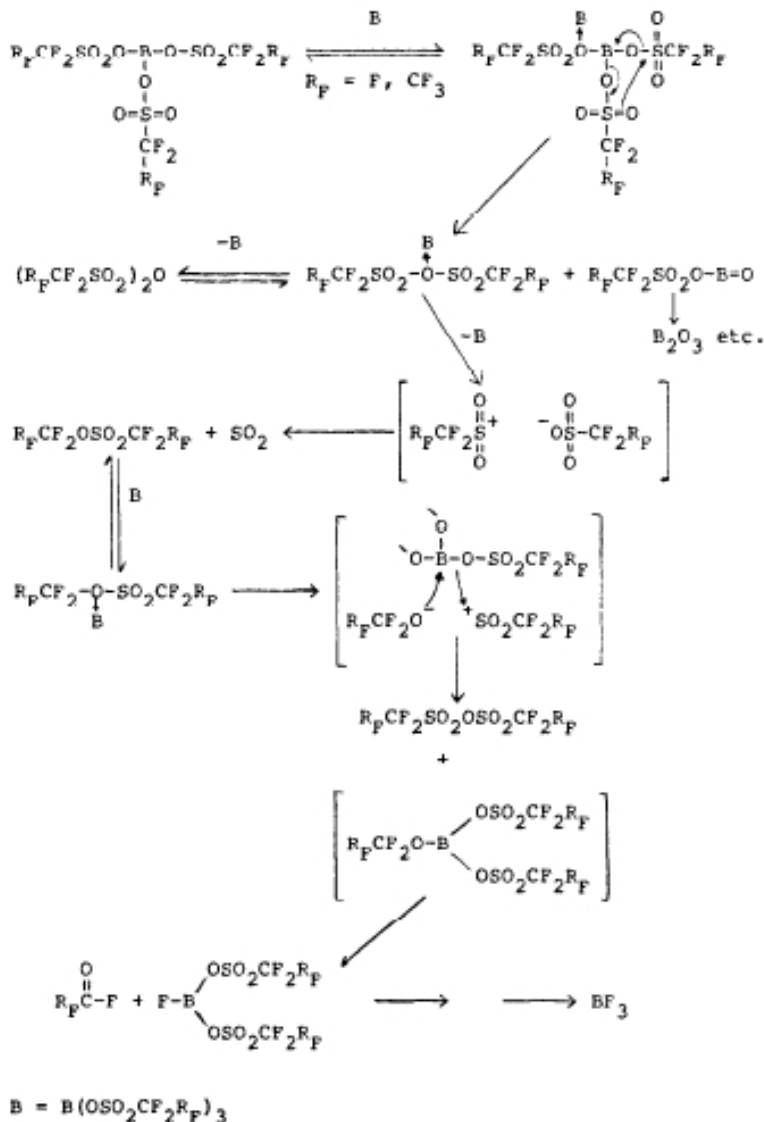
Fig. 20. Proposed mechanism for thermal degradation of tris trifluoromethane sulfonate (triflate) 3 .
