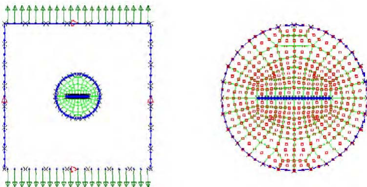
Figure 8: Circular composite patch over a cracked square sheet: BEM model
