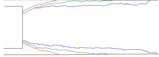
Figure 3. Representative profiles of a long, medium and short film. These profiles are from the geometry shown in Fig. 2 at momentum flux ratios of 110, 484 and 823 respectively
