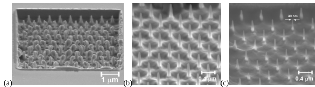
Figure 5: (a) as-milled nanopillar array (b) nanopillars after brief KOH etching (c) nanopillars of smaller size (~30nm) after further KOH etching
