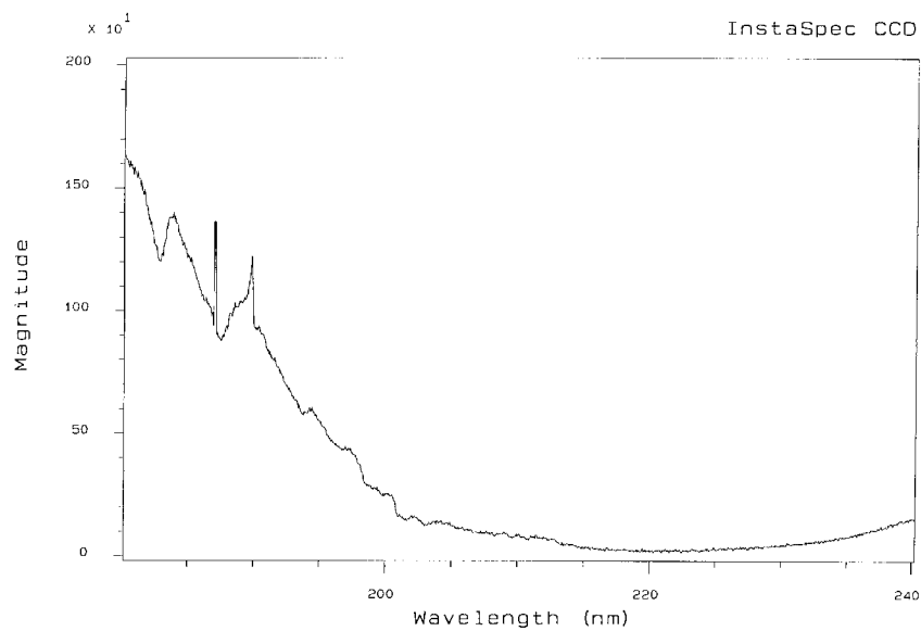
UV SPECTRA
