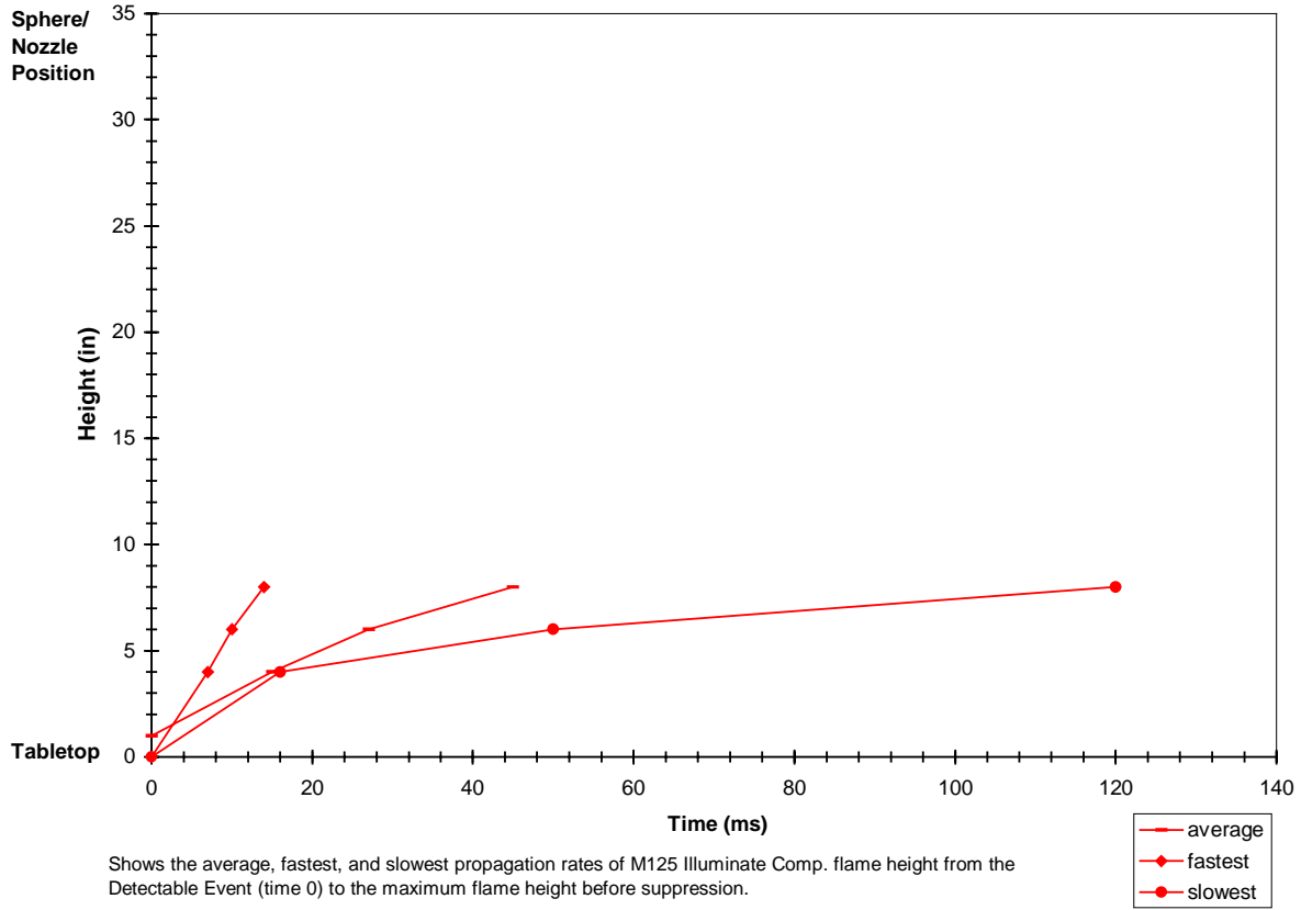
M125 Illuminate Comp. Propagation Rates
