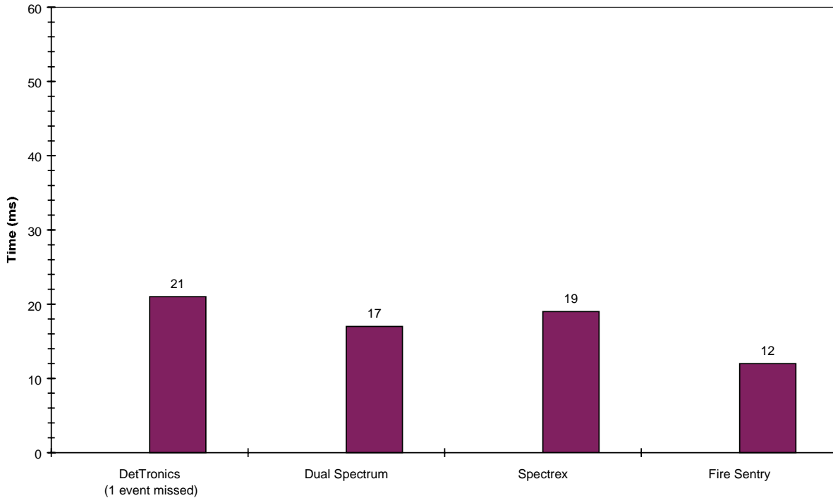
Average Response Times to Red Lead
