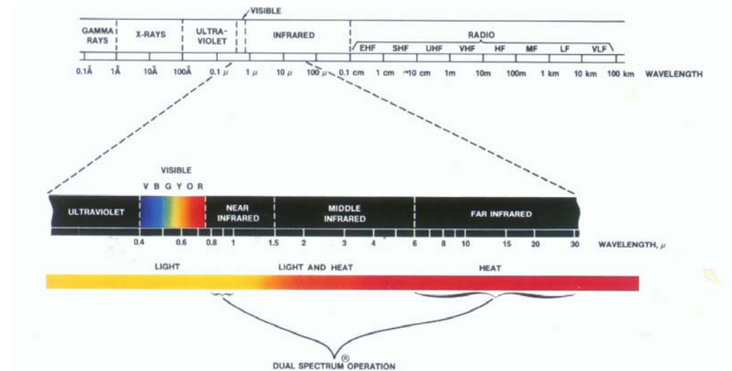
TYPICAL HYDROCARBON FIRE EMISSION SPECTRUM SHOWING DETECTION REGIONS OF OMNIGUARD 730
