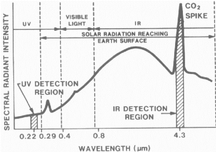
TYPICAL HYDROCARBON FIRE EMISSION SPECTRUM SHOWING DETECTION REGIONS OF OMNIGUARD 730
