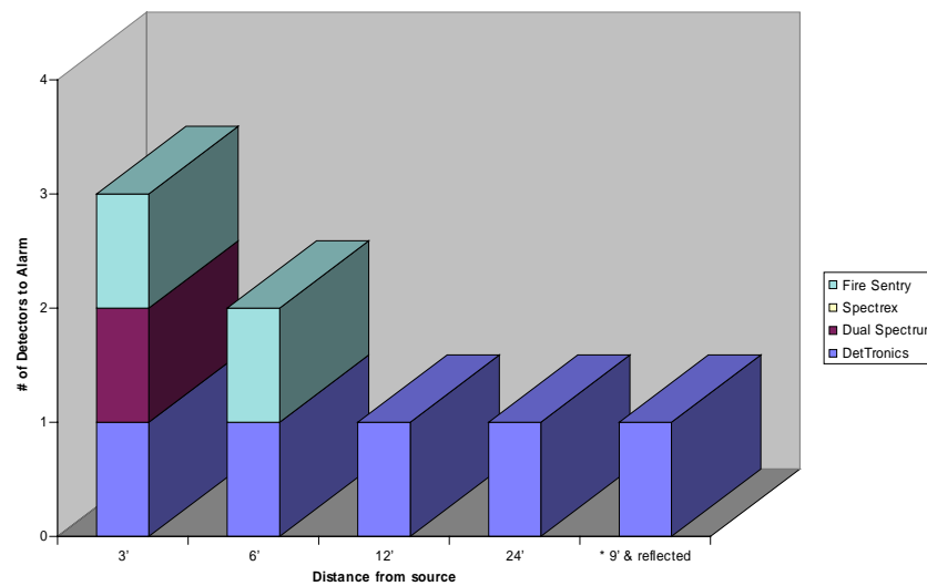
Arc Welding (6011 1/8" rods, mild steel, 104 A)
