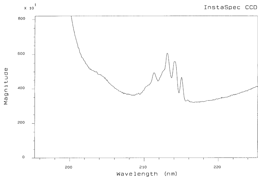
UV SPECTRA
