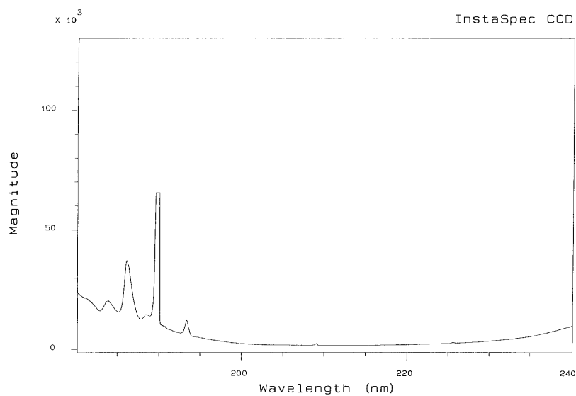
UV SPECTRA
