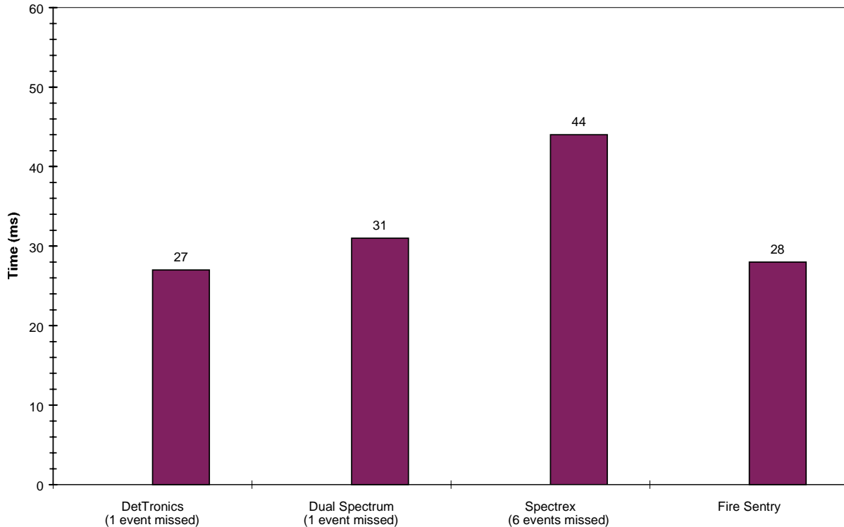
Average Response Times to MK25 Starter Comp.
