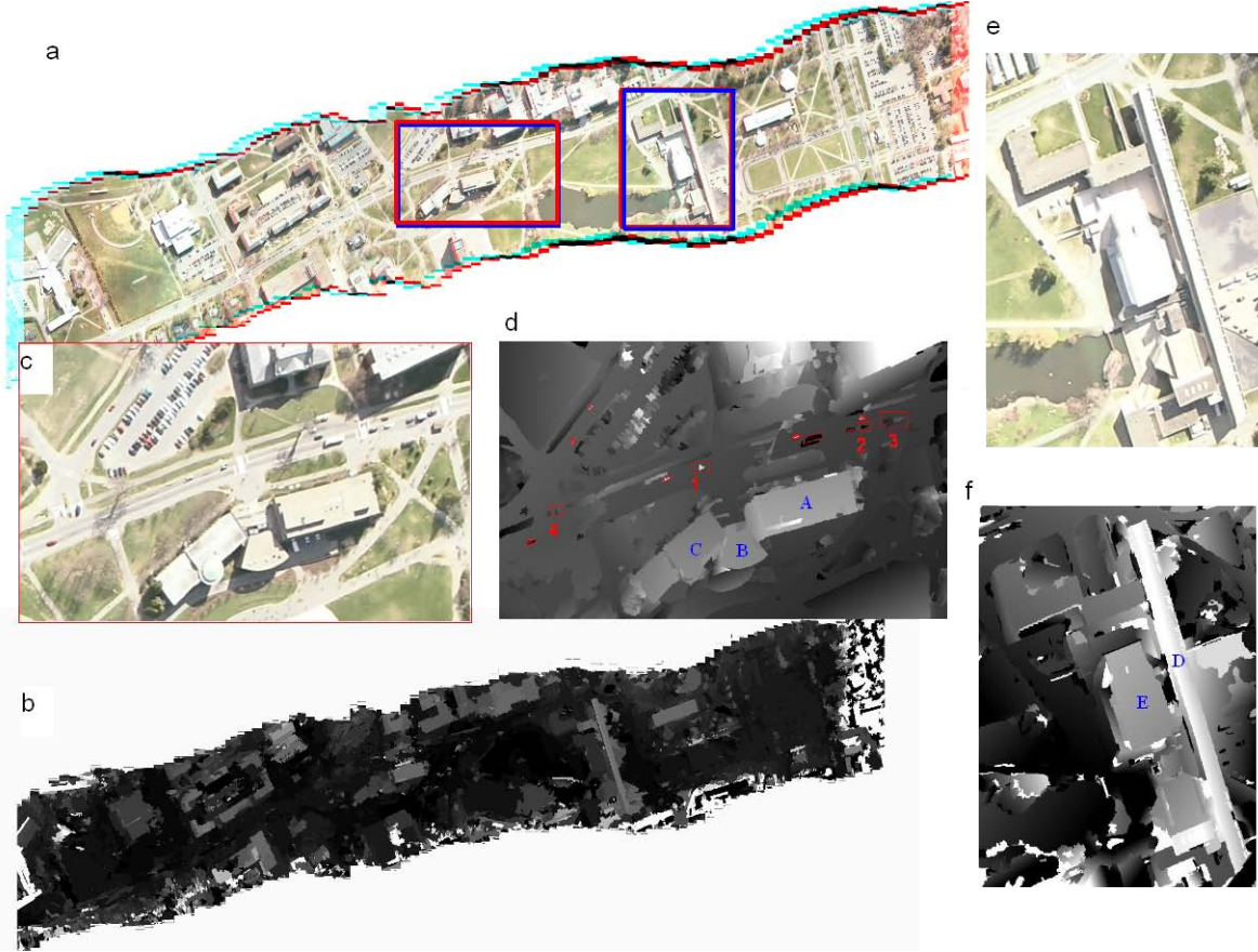
Fig. 12. 3D and motion from multi-view stereo mosaics of an aerial video sequence. (a) A pair of stereo mosaics from the total nine mosaics; (b) height map of entire mosaic; (c) close-up of the 1 st window marked in (a); and (d) the height map of the objects inside that window, with the detected moving targets marked by their boundaries and those not detected by rectangular boxes; (e) close-up of the 2 nd window marked in (a); and (f) the height map of that window.
