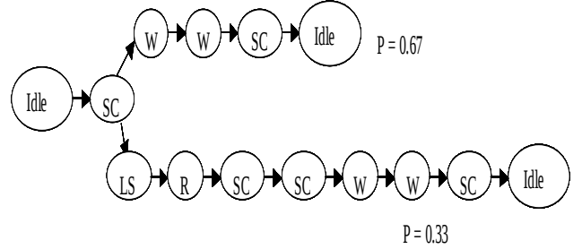
Figure 2. Stochastic State-Transition Graph Representing Two Scenarios in an Active Application (System Calls: LS = _llseek ; R = read; SC = socket call; W = write) (P = the probability of executing a specific scenario)
