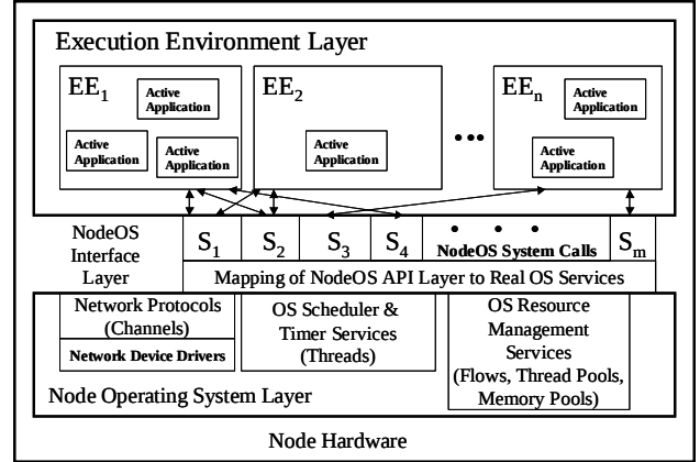
Figure 1. Conceptual Architecture of an Active Network Node
