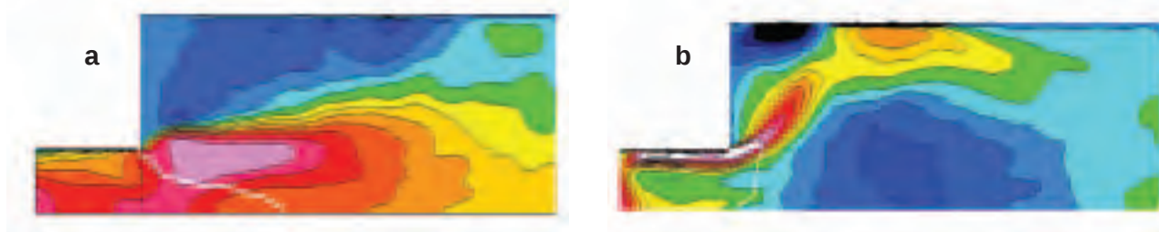
Figures 1a and b. Isocontours of axial velocity in the combustor for two different swirl numbers (left S = 0.56 , right S = 1.12 ). The colors red and green indicate left-to-right flow, whereas blue and black indicate reverse flow. As shown, increase in swirl creates a recirculating (reverse flow) bubble in the combustor that pushes the flame outward and also stabilizes the combustion.
