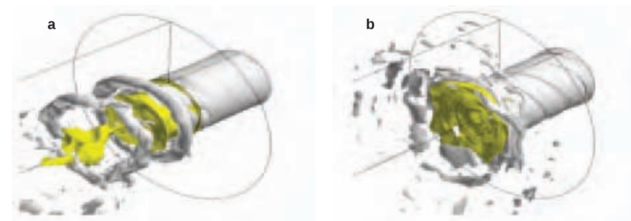
Figures 2a and b. Increase in swirl (left to right) in a premixed system stabilizes pressure oscillation in a gas turbine and also directly impacts the flame (yellow)-vortex (gray) interaction process. With high swirl, the shear layer at the dump plane breaks down, and a recirculation bubble forms in the combustor that stabilizes the flame; hence the combustion process.
