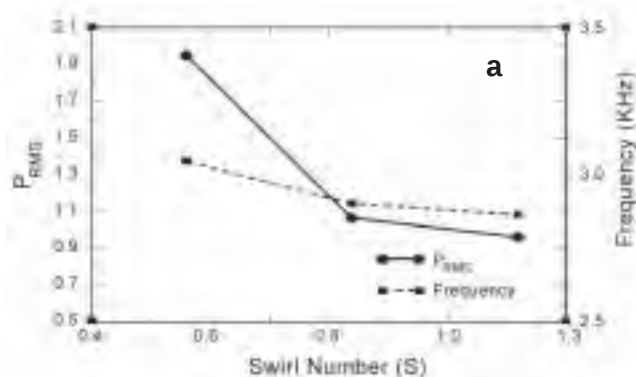
Figures 3a and b. The effect of increasing swirl (for a fixed equivalence ratio) is to decrease the pressure oscillation amplitude and the effect of decreasing equivalence ratio (for a fixed swirl) is to increase the pressure oscillation amplitude. Data such as this can be used to devise an active swirl control strategy.
