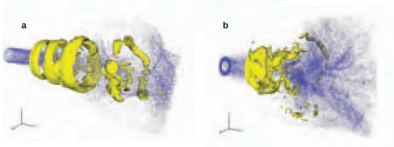
Figures 4a and b. Increase in swirl (left to right) also can be used to control the spray dispersion into the combustor. This in turn directly controls the combustion process in the combustor. Spray dispersion is increased in high swirl because of the breakdown of the vortex structures, which enhances local entrainment, and the formation of the recirculation bubble, which provides an effective bluff body to push the spray droplets around it and hence increase dispersion. The combustion efficiency (not shown) is also increased with an increase in swirl.
