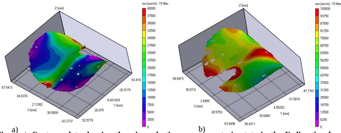
Fig. 5. Contour plots showing the wings elastic membrane strain state in the X direction for wind-off conditions. The strains are: low-tension case (left) and high-tension case (right). The values are in microstrain ( \mu\text{m}/\text{m} ).
