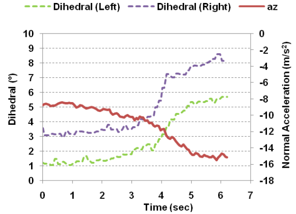
Figure 13. Time history of the correlation between the normal acceleration and the wing dihedral during a roll doublet.
