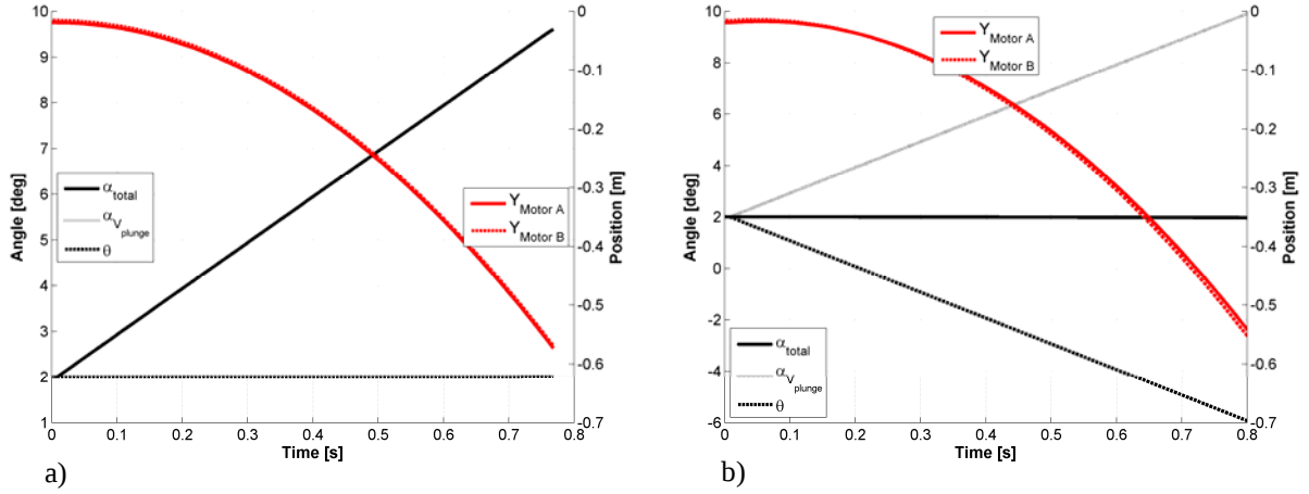
Figure 4. Combined plot with model angle of attack, pitch angle, and motor position versus time. Left) \dot{\alpha} = 10^\circ/s case (pure plunge). Right) \dot{\theta} = 10^\circ/s case (pitching/plunging). The position of the model is displayed in red on the right axis.
