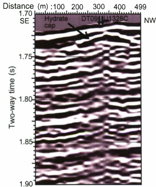
Figure 10. Southeast-northwest seismic section, showing hydrate cap details from Teledyne 2000 crossline XL75 (see Figure 2 for location). The locations of intersection with DTAGS line DT09 and nearby IODP site U1328 are also labeled. Note reduced seismic amplitudes below the hydrate cap (center of the vent).
