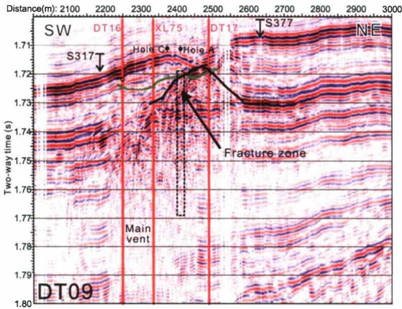
Figure 13. Southwest-northeast seismic section from DTAGS2 line DT09. The green curve is the hydrate cap location indicated from the Teledyne 2000 grid; the black curve is from the DTAGS line. The dashed black rectangle box indicates a layer with high hydrate concentrations from about 540 mbsf revealed by the resistivity log of IODP site 1328 hole A on this line (Figure 15). The top of this layer corresponds to the hydrate cap location. Maximum hydrate concentrations (~60%) correspond to a high-reflectivity fracture zone that projects to the seafloor. The two locations where velocity analyses were applied are also labeled (S317, S377).
