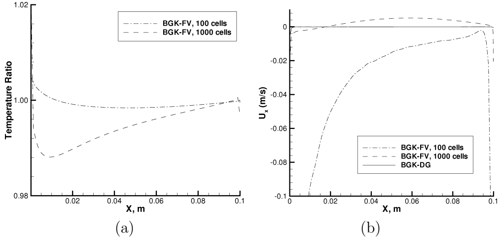
Figure 9: FV to DG temperature ratio (a) and gas flow velocity (b), for heat transfer problem at Kn=0.01 .
