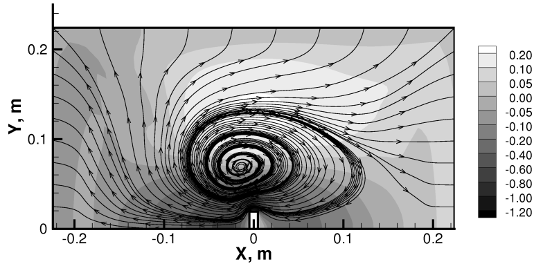
Figure 1: Flow velocity and streamlines around a radiometer vane in a 6 Pa argon gas, obtained by a finite volume approach to the BGK equation.
