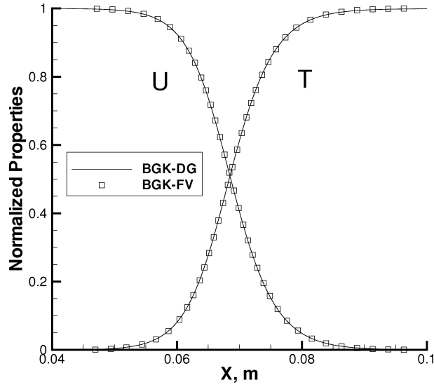
Figure 2: Normalized velocity and temperature in a Mach 1.2 shock wave. Comparison between the DG and FV approaches.
