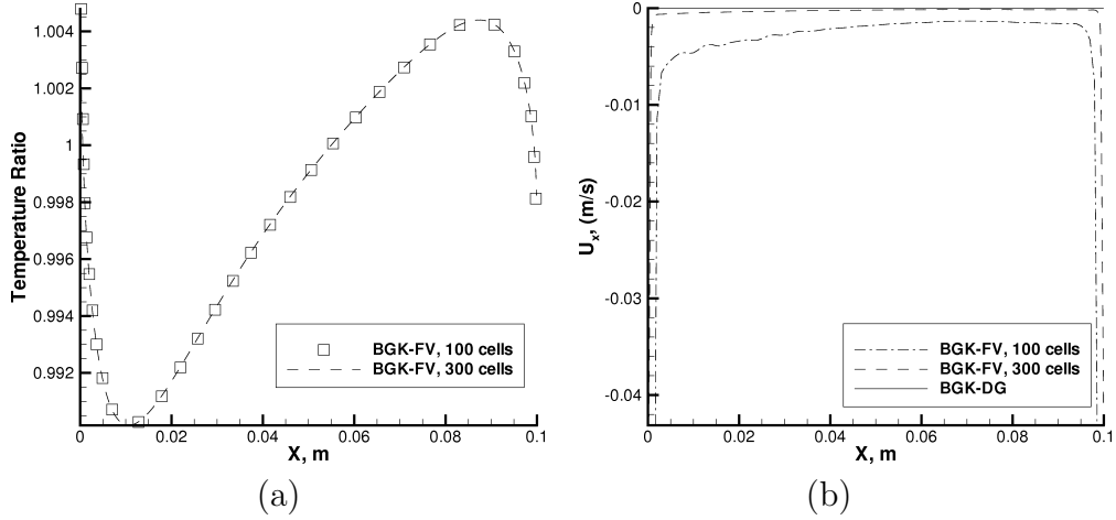
Figure 8: FV to DG temperature ratio (a) and gas flow velocity (b), for heat transfer problem at \text{Kn}=1 .
