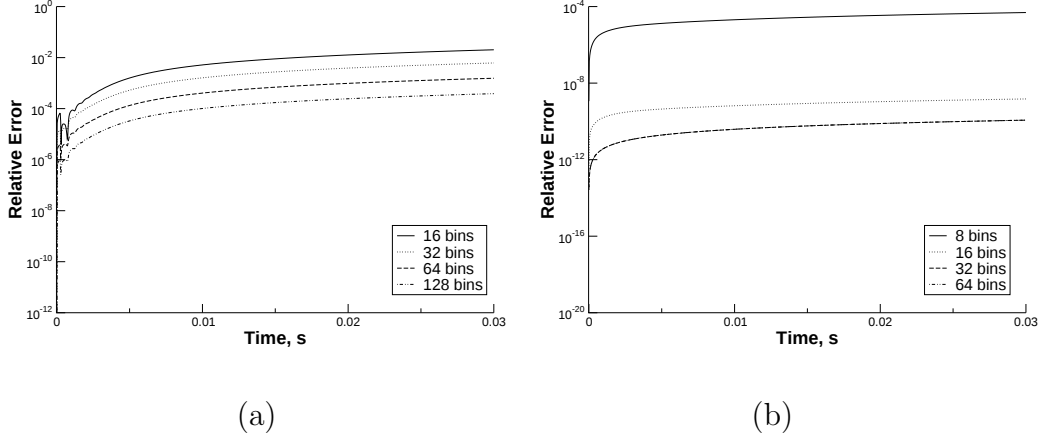
Figure 5: Convergence of relative error in the total mass with respect to the resolution in velocity space. Comparison of (a) fourth and (b) eighth degree polynomial approximations.
