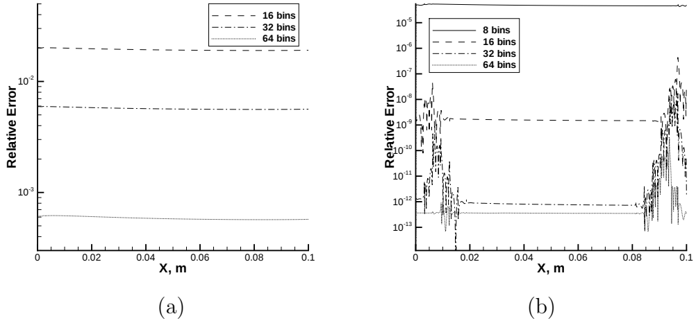
Figure 6: Convergence of the solution in a Kn=0.01 heat transfer problem as a function of the number of velocity bins. Comparison of (a) fourth and (b) eighth degree polynomial DG approximation in velocity space.
