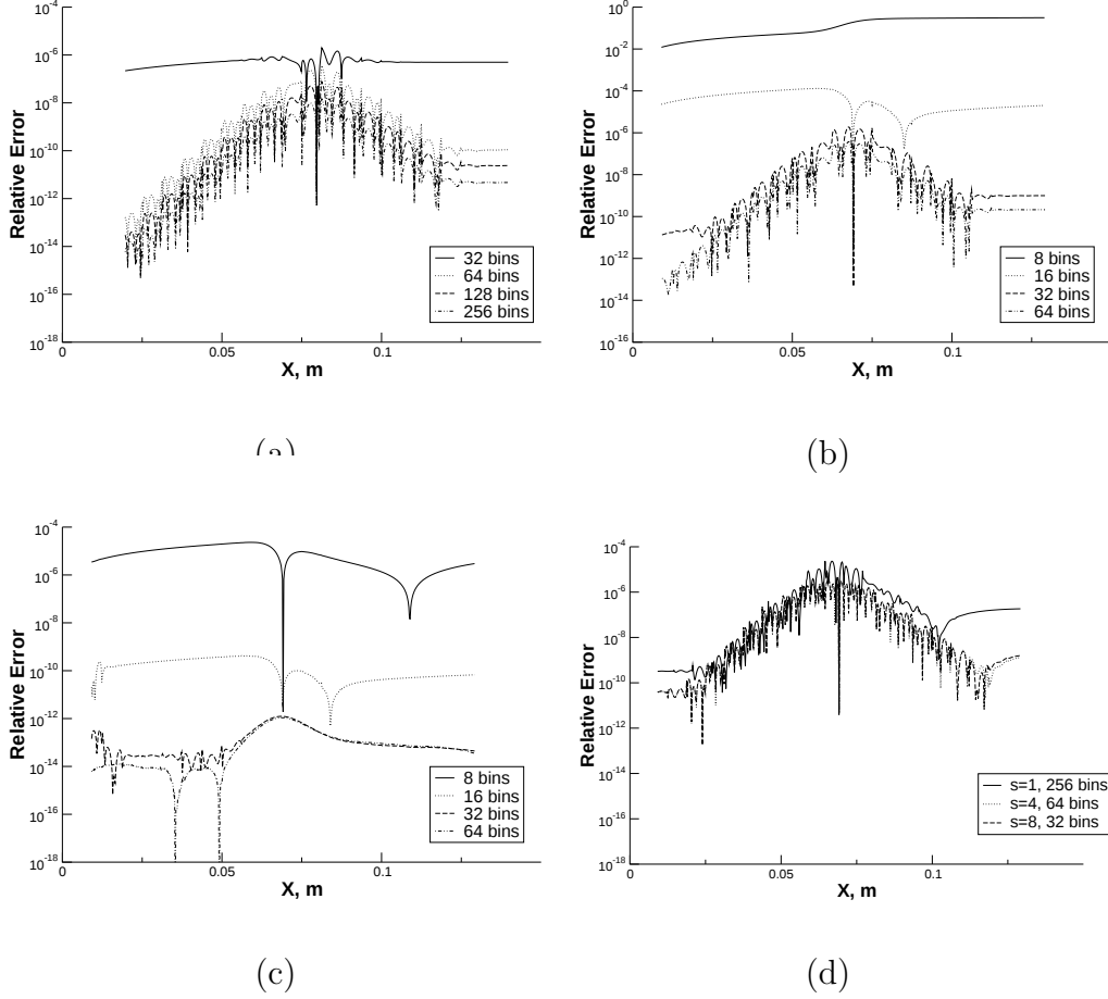
Figure 3: Convergence of the DG solution in a Mach 1.2 shock wave as a function of the number of velocity bins. Comparison of the DG discretizations by (a) first, (b) fourth and (c) eighth degree polynomials. In figure (d) solutions on 32 spatial cells are compared to a solution on 64 spatial cells.
