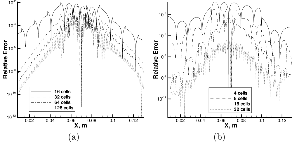
Figure 4: Convergence of density in a Mach 1.2 shock wave as a function of spatial cells. Comparison of (a) second and (b) fifth order DG discretizations.
