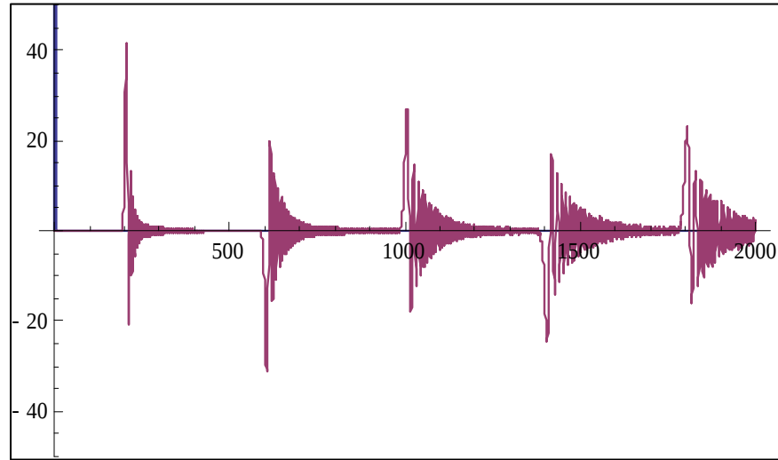
Figure 12. Low voltage response to figure 11 test pulse at end of NLTL.
