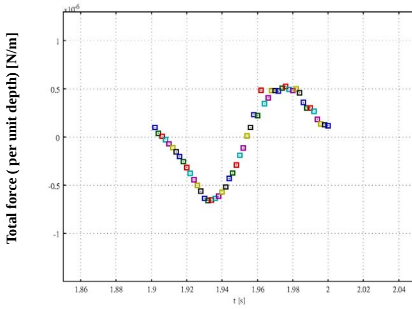
Figure 9e. Time excursion of the integrated force on the entire structure for (\delta = 0.5t; f= 10\text{Hz}) . Due to the presence of extrusions, asymmetry in the time variation is shown, unlike that for the purely flat plate case. At this low frequency, the total force (per unit depth) is -1.14\text{e-}8 \text{ N/m} – not very significant still.
