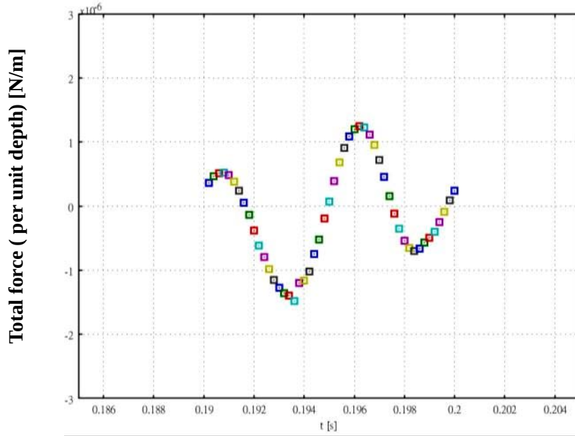
Figure 8d. Time excursion of the integrated force on the entire structure for increased amplitude ( \delta = 0.1t ; f = 100\text{Hz} ). Due to the presence of extrusion, asymmetry in the time variation is shown, unlike that for the purely flat plate case. The total force (per unit depth) is -1.17\text{e-}7 \text{ N/m} – not very significant.
