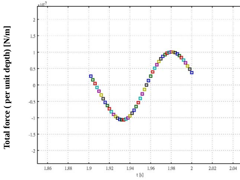
Figure 9c. Time excursion of the integrated force on the entire structure for ( \delta = 0.1t ; f = 10\text{Hz} ). Due to the presence of extrusions, asymmetry in the time variation is shown, unlike that for the purely flat plate case. At this low frequency, the total force (per unit depth) is -5.54\text{e-}10 \text{ N/m} – not very significant.
