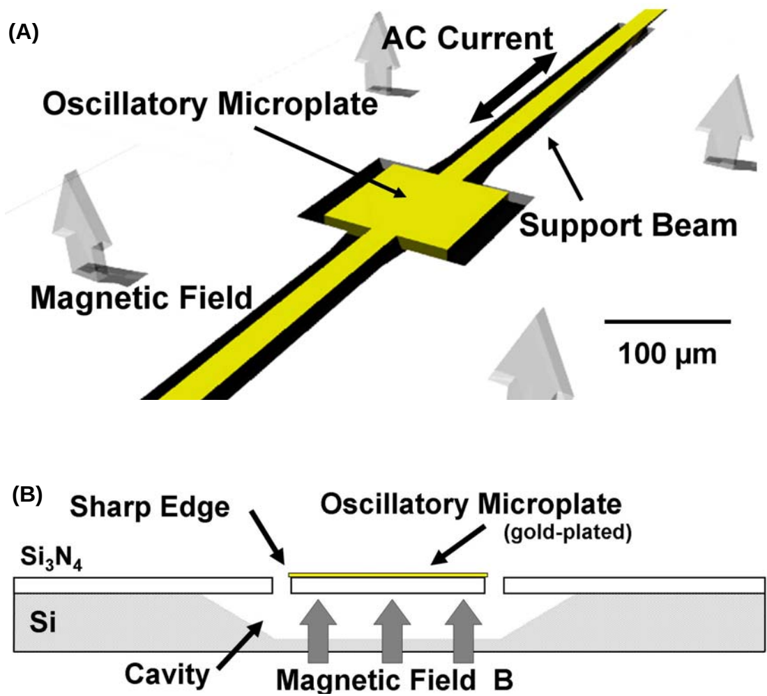
Figure 1. The microdevice. (A) Suspended microplate (100*100*1 \mu\text{m} thick) in resonance (140kHz). Plate oscillation is due to Lorentz induced force from AC current flows through the structure above an external magnetic field. (B) Edge-on view showing sharp edges of the microplate, 20 \mu\text{m} spacing between microplate and fixed \text{Si}_3\text{N}_4 structure, cavity underneath, and material details.
