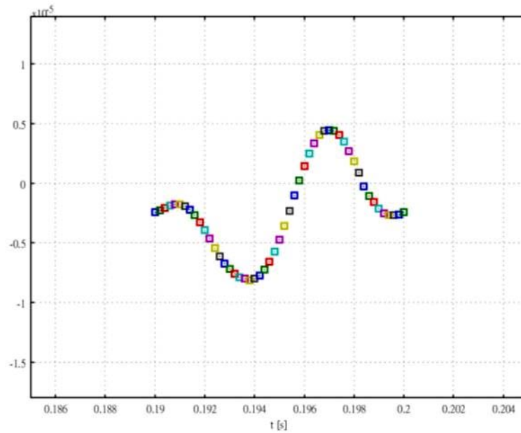
Figure 9f. Time excursion of the integrated force on the entire structure for (\delta = 0.1t; f= 100\text{Hz}) . Due to the presence of extrusions, asymmetry in the time variation is shown, unlike that for the purely flat plate case. At this low frequency, the total force (per unit depth) is -2.26\text{e-}6 \text{ N/m} .
