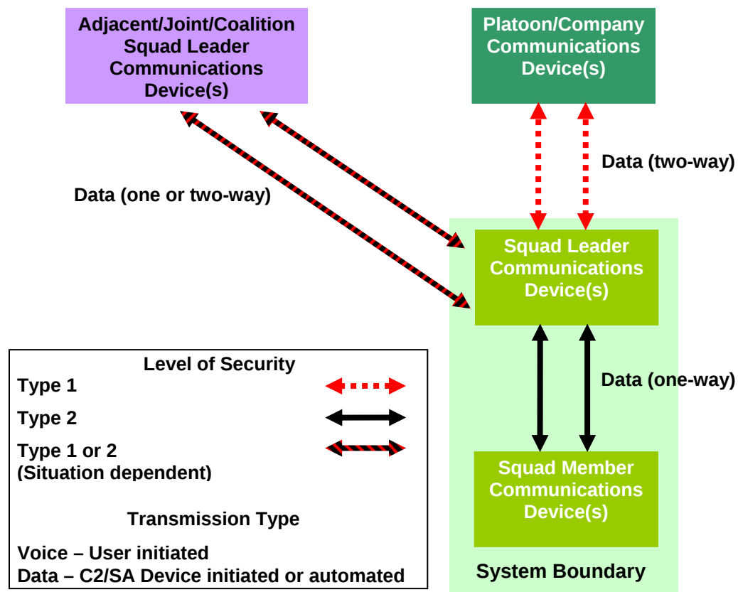
Figure 4: Communications System Context Diagram
