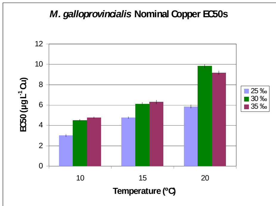
Figure 2. Mean control performance ( \pm 1 s.d.)(top figure) and EC50 values ( \pm 95\% C.L.) (bottom figure) for mussel ( Mytilus galloprovincialis ) embryo-larval development following 48–72 h exposures in clean or copper-spiked seawater under varying salinity and temperature combinations (from Burton et al. 2008).
