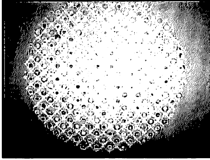
Figure 1. Waffle mode over a DM. An interferogram over a DM is shown with the actuators commanded to the waffle pattern.
