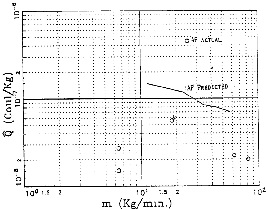
Figure 10 AP predicted vs. actual charge density readings. The solid line represents the maximum predicted charging expected during AP feeding. * The feed system was clean before this run.
