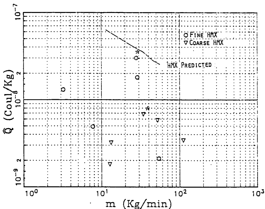
Figure 11 HMX predicted vs. actual charge density readings. The solid line represents the maximum predicted charging expected during HMX feeding. * The feed system was clean before this run.
