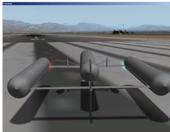
Figure 13. UAV with three motor nacelles.
