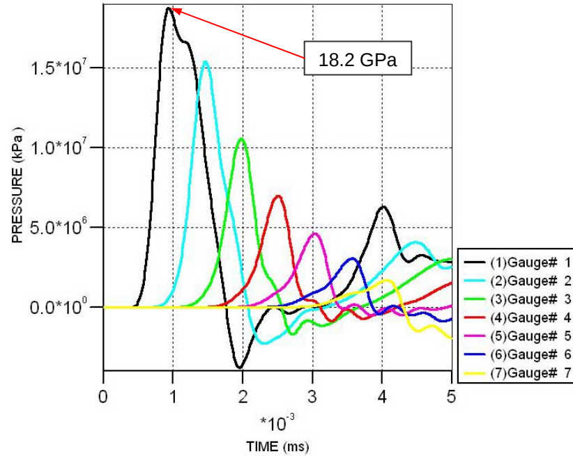
Figure 17. Pressure Versus Time Plot of Tantalum Target Plate
