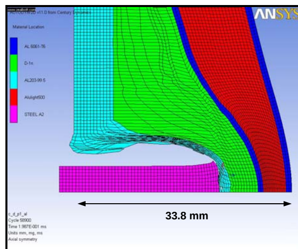
Figure 47. Simulation Results of Shot Number 12
