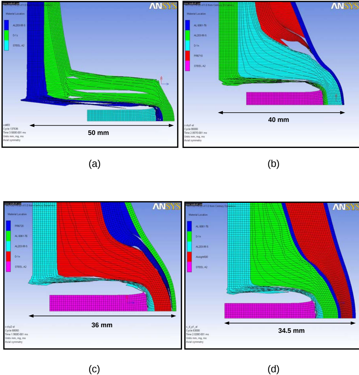
Figure 49. Simulation Result of a 1" Steel Rod Projectile Impacting (a) C-D; (b) C-D-P1-Al; (c) C-D-P2-Al and (d) C-D-M Target Plate at 483 m/s
