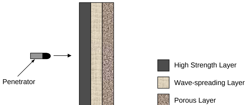
Figure 1. Multi-layered Structure Armor Concept
