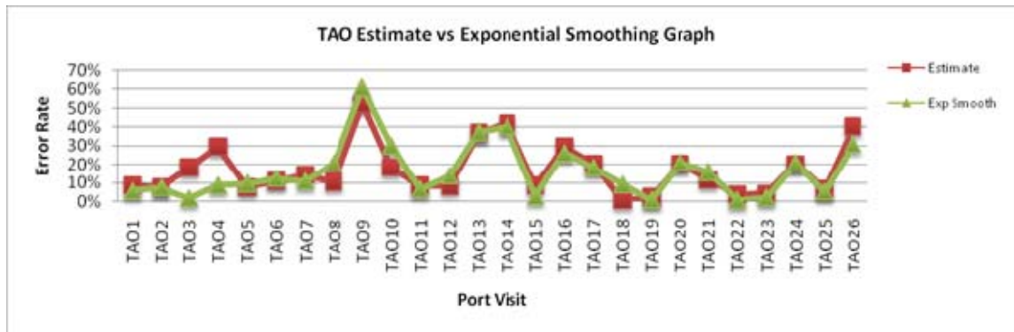
Figure 26. Graph of 2008–2009 TAO Estimate and Exponential- smoothing Error Rate.
