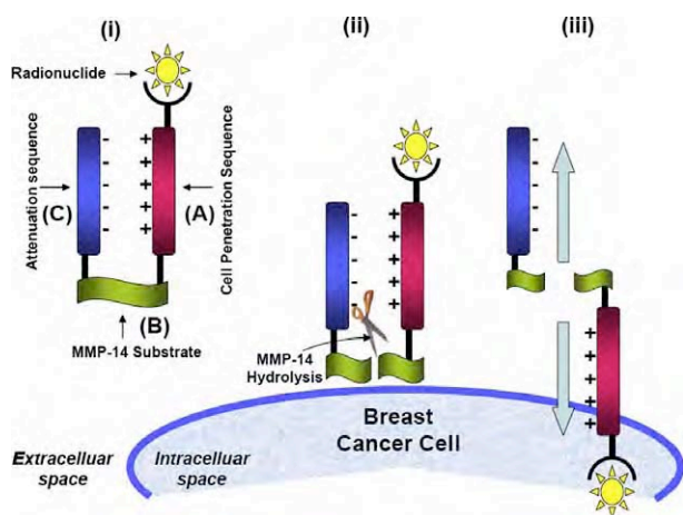
Figure 1. Outline of the probe structure and mechanism. The quenched probe (I) is able to freely circulate in vivo , until it encounters its protease target. Cleavage of the probe at a defined point by MMP-14 (II) releases a cell penetrating peptide, which can then translocate its radionuclide cargo across the target cell membrane (III). After uncleaved quenched probe is washed away, the internalized radioactivity can be imaged by SPECT.
