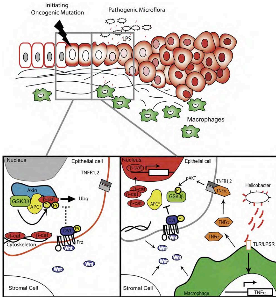
Figure 1. Macrophage-Derived TNF \alpha Activates Wnt/ \beta -Catenin during Gastrointestinal Cancer Development
