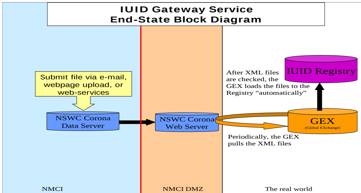
Figure 8. Gateway Between NMCI and the DoD UID Registry (From MacDougall & Pompa, 2009)
