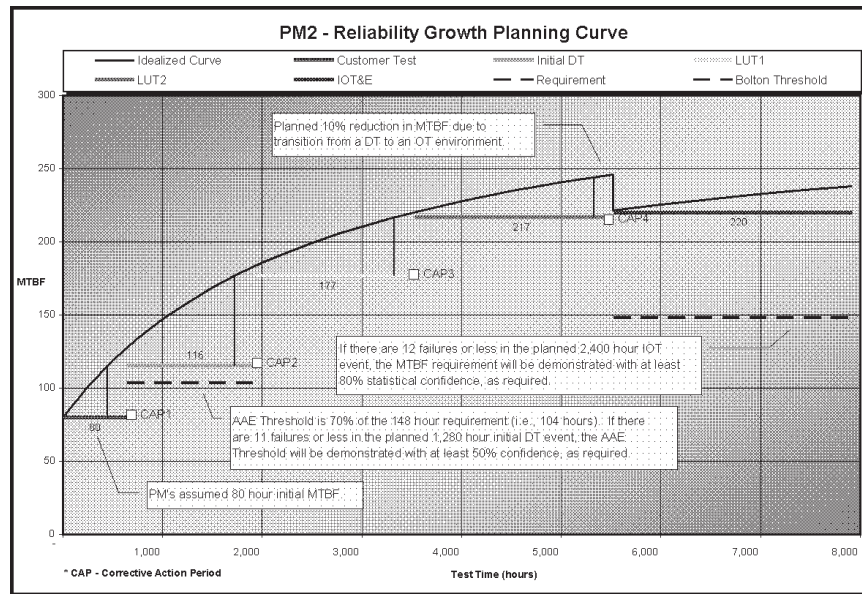
Figure 6. Reliability growth planning curve
