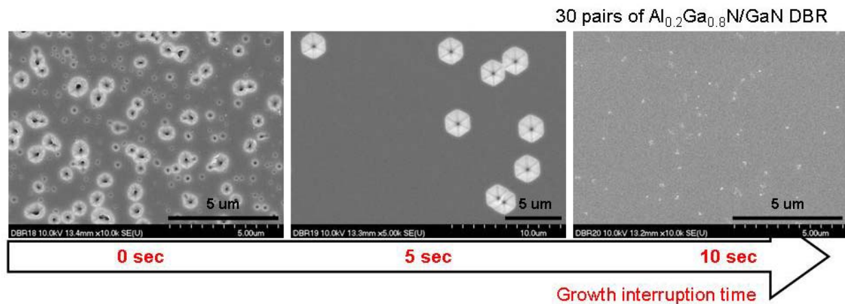
Fig. 10. SEM images of 30 pairs of \text{Al}_{0.2}\text{Ga}_{0.8}\text{N}/\text{GaN} DBR structure with growth interruption time
