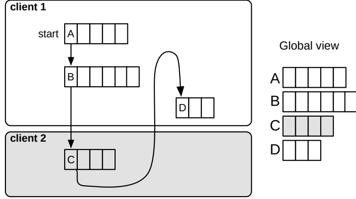
Figure 4: Logs of nested distributed transactions
