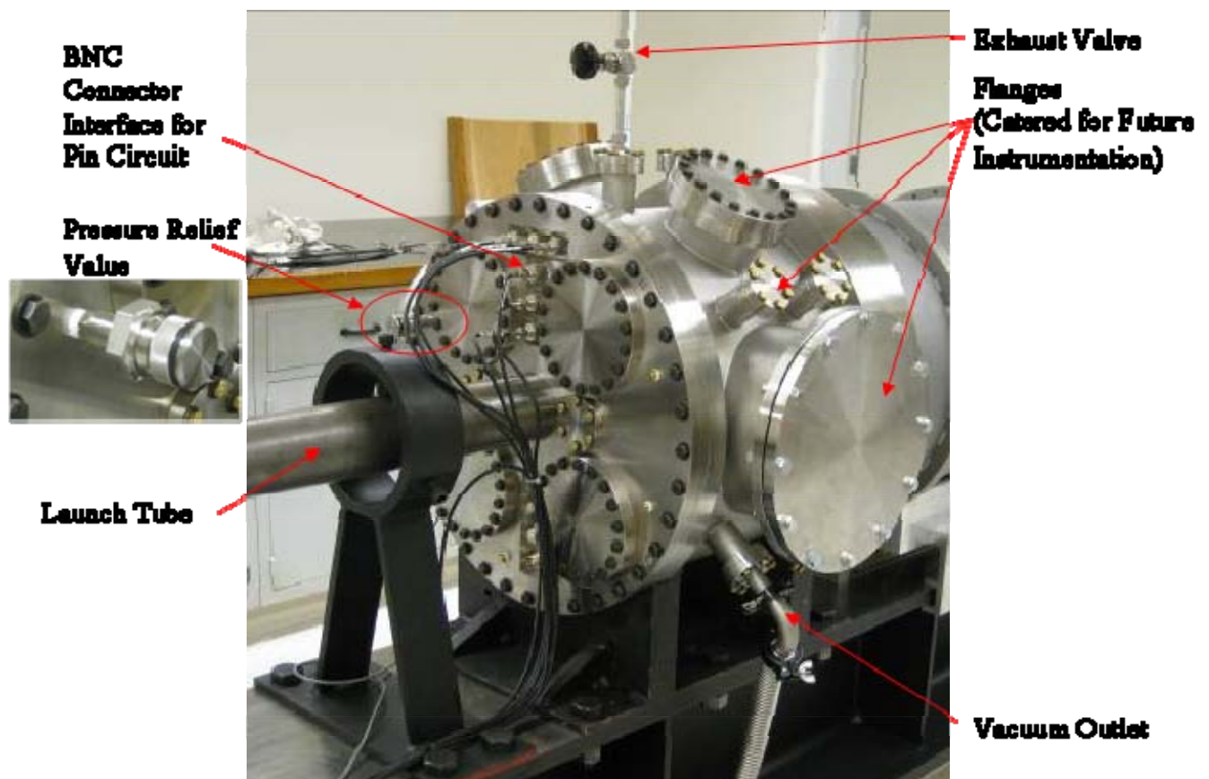
Figure 15. Diagnostic Tank
