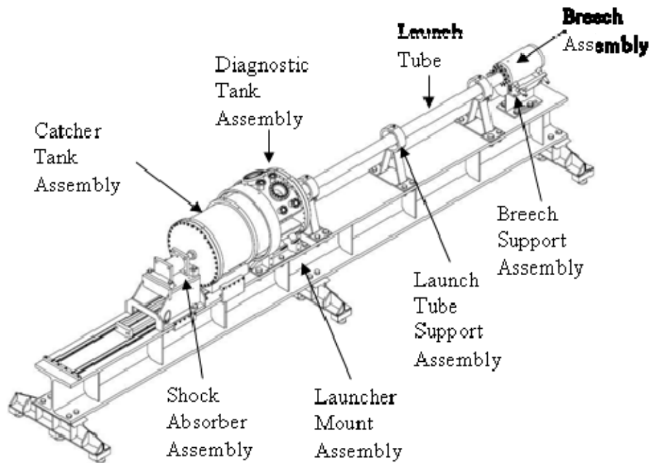
Figure 7. Main Gas Gun Assembly [After 5]
