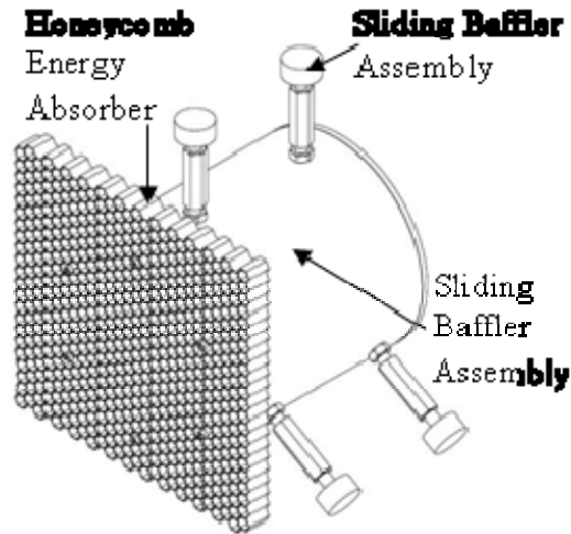
Figure 18. Sliding Baffler Assembly [After 5]
