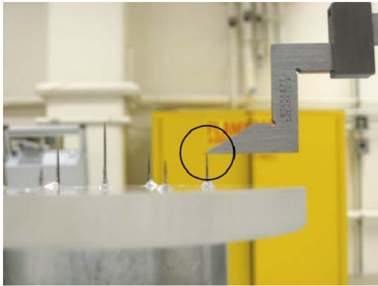
Figure 39. Venire in Contact with Pin for Measurement
