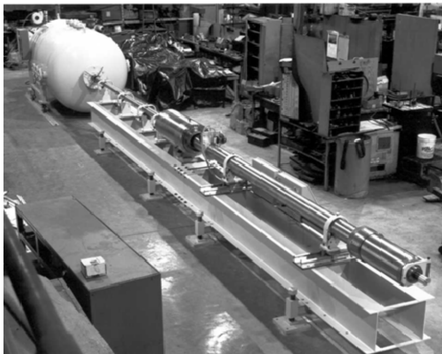
Figure 5. Propellant and Gas-driven Gas Gun [1]
