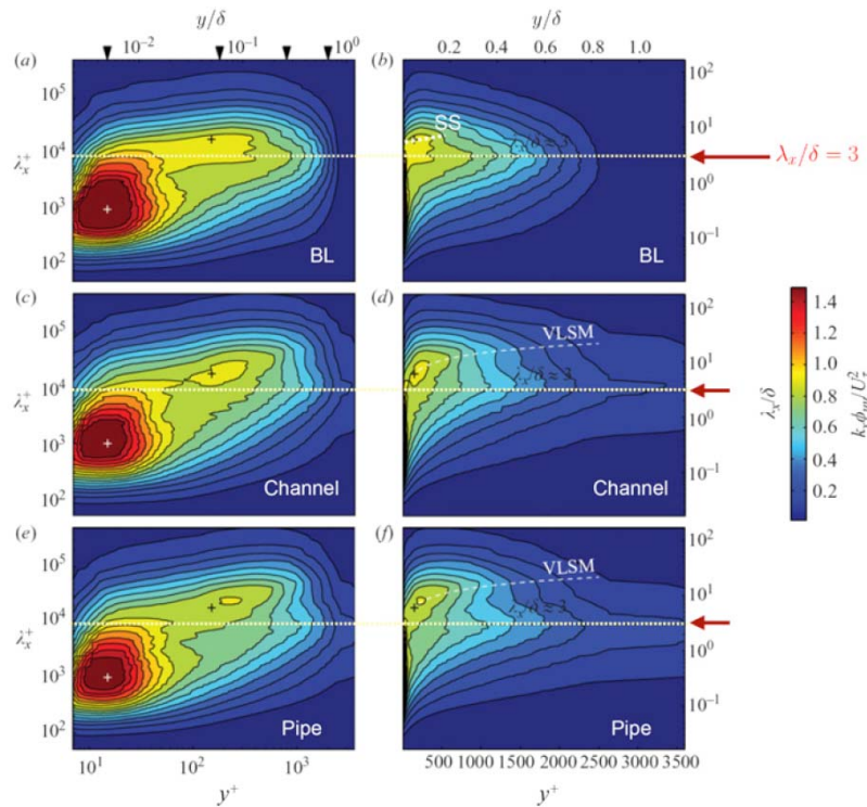
Figure 2: Maps of premultiplied u spectra as a function of streamwise wavelength \lambda_x and distance from the wall. Figures show (from top to bottom) turbulent boundary layer (a, b), channel (c, d) and pipe (e, f), respectively. Right-hand figures have a linear abscissa, to emphasize the differences in the outer region between VSLM in pipes and channel and the superstructures in boundary layers. Red arrows indicate the wavelength \lambda_x / \delta = 3 .
