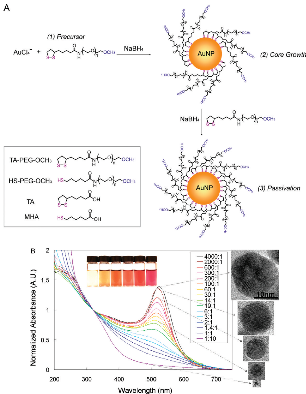
Figure 1. (A) Schematic representation of the one-phase growth method using TA-PEG-OCH 3 ligands. (B) Normalized UV–vis absorption spectra for several Au/ligand molar ratios used for the growth (of AuNPs with different sizes), along with a few representative TEM images collected for selected subsets of these nanocrystals. (inset) Image collected from a series of AuNP dispersions in deionized water. Changes in solution color from light to dark brown and to red (from left to right) reflect increase in AuNP size.
