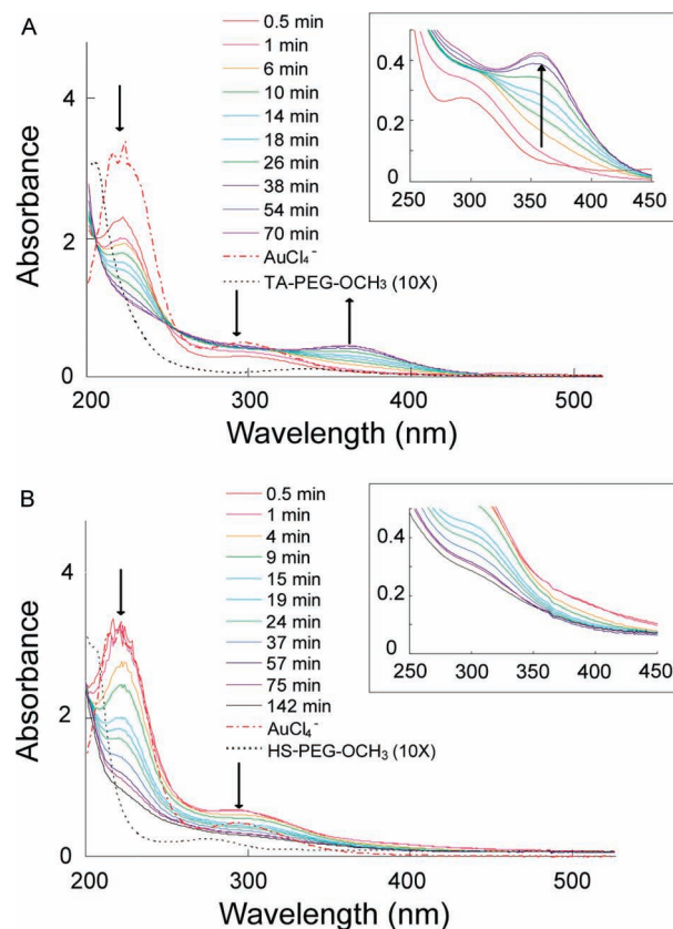
Figure 6. Time-dependent UV-vis absorption spectra for HAuCl 4 and ligand mixtures (Au/ligand = 3:1, concentration of ligand = 106 \mu M). (A) TA-PEG-OCH 3 and (B) HS-PEG-OCH 3 . Changes in the spectra are indicative of ligand to gold complex (precursor) formation. The spectra for other ligands including TA and DHLLA-PEG-OCH 3 are provided in the Supporting Information. Excess of 10 \times corresponding to 1.06 mM was used for the pure ligands.
