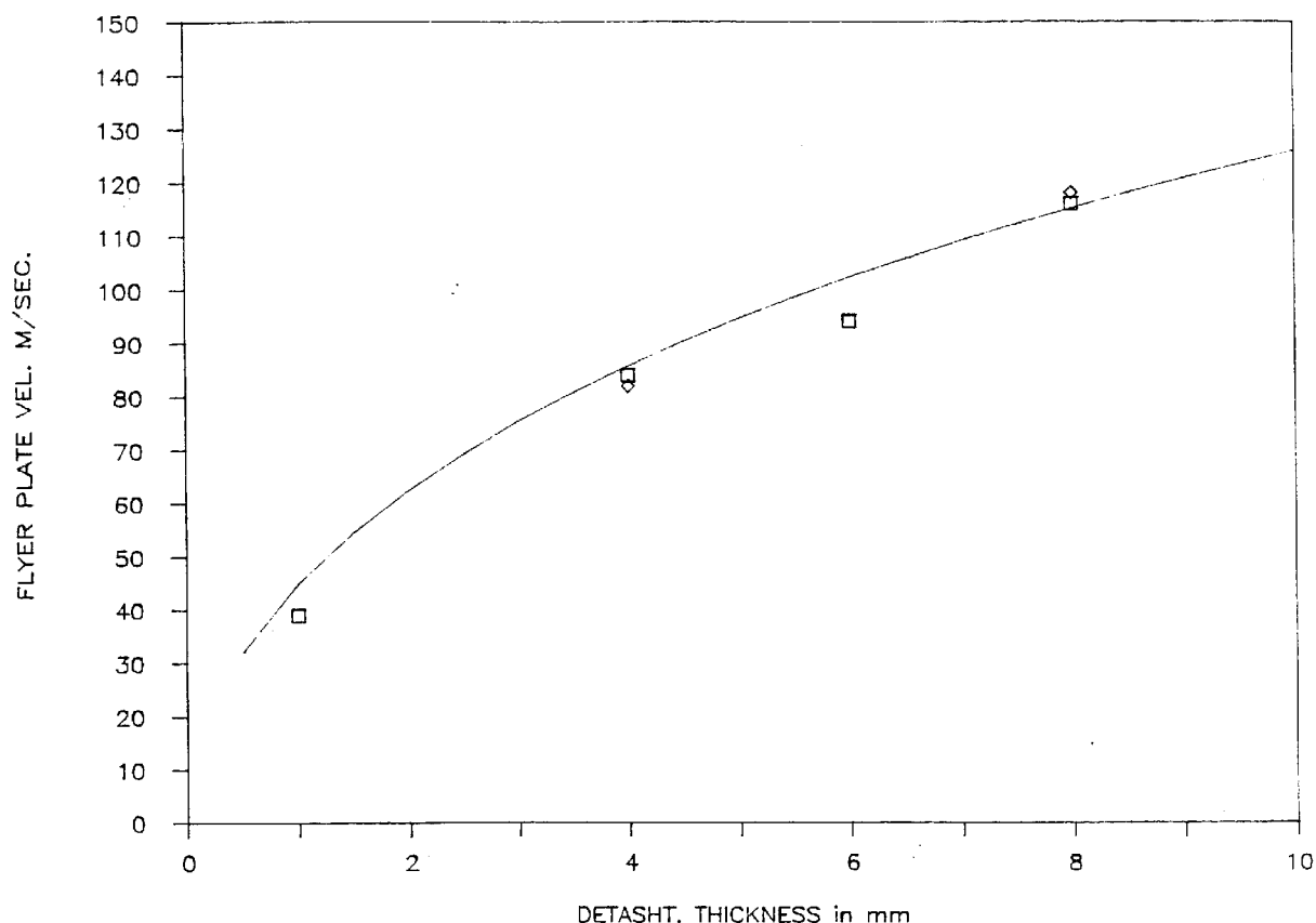
Figure 10. Flyer plate (4-in) velocity vs. Detasheet thickness (for 1-in thickness of steel tamper).
