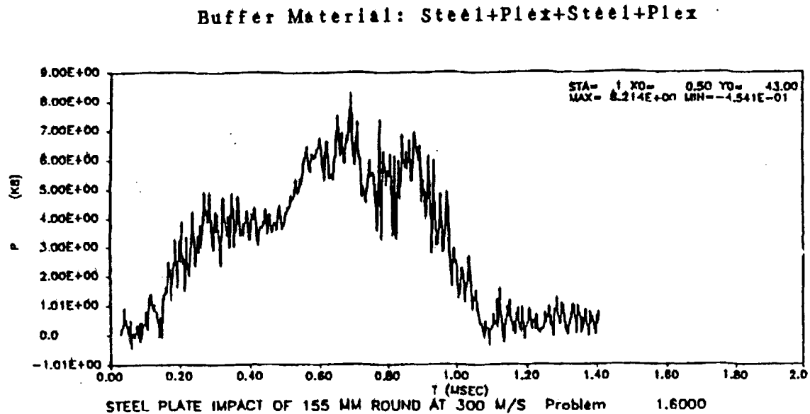
Figure 2. Computed pressure as a function of time for layout in Figure 1 at station No. 1. (Time is in milliseconds; Pressure is in kilobars. Plate velocity was 300 m/s.)
