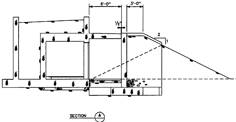
FIGURE 2 - CROSSECTION
