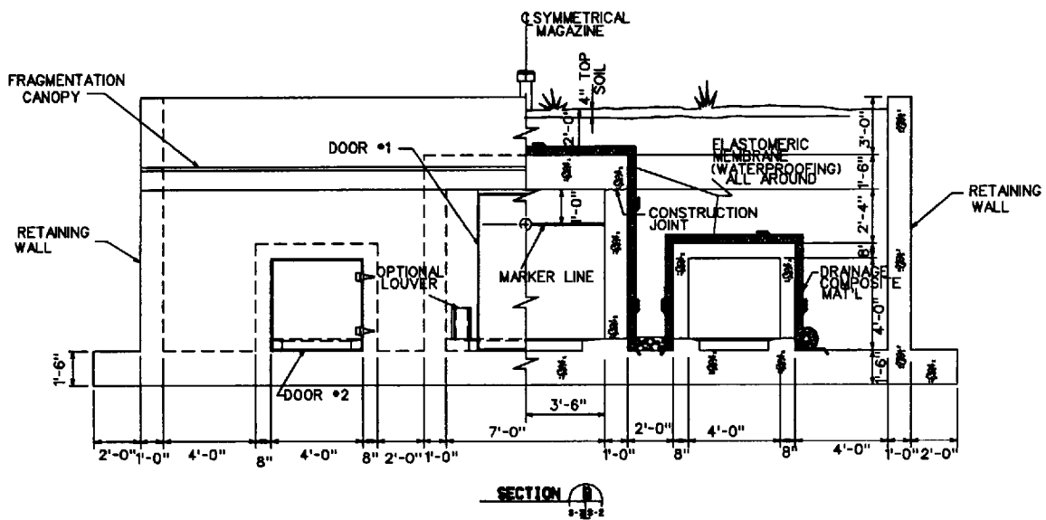
FIGURE 4 - SECTION THROUGH CHAMBERS
