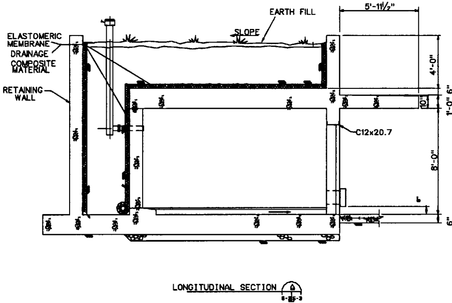
FIGURE 8 - DETAILED CROSS-SECTION
