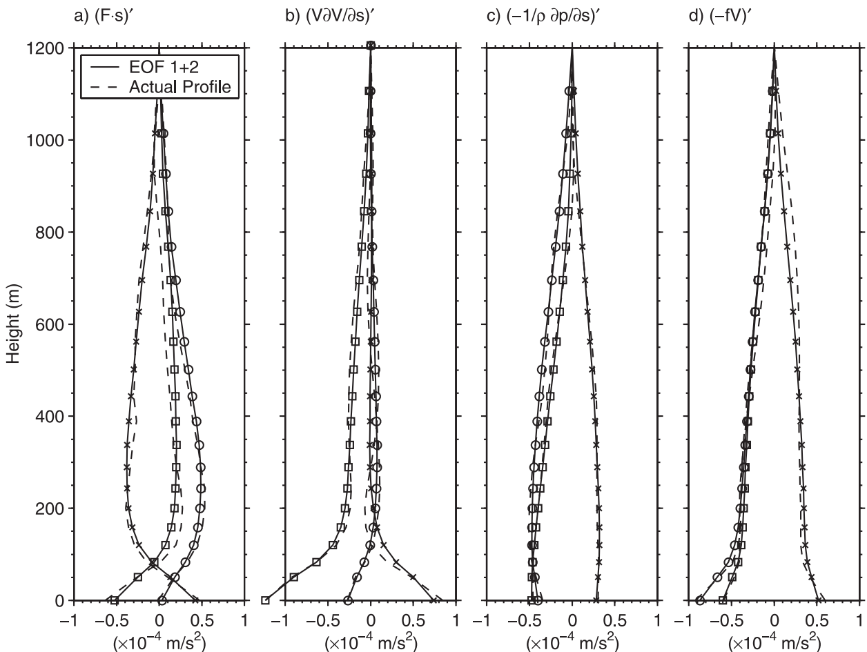
FIG. 8. Vertical profiles of select 1-month-averaged forcing terms in the WRF momentum budget at three different points (dashed) along with the EOF representation of these terms computed from the first two modes (solid). Four terms are chosen: (a) downwind turbulent stress divergence (\mathbf{F} \cdot \mathbf{s})' ; (b) downwind horizontal advection (V\partial V/\partial s)' ; (c) downwind pressure gradient [-(1/\rho)(\partial p/\partial s)]' ; (d) Coriolis force (-fV)' . The three locations chosen are 44^\circ\text{S} , 61^\circ\text{E} (crosses; cool to warm); 44.5^\circ\text{S} , 65^\circ\text{E} (circles; SST minimum); and 42.2^\circ\text{S} , 68^\circ\text{E} (squares; warm to cool).
