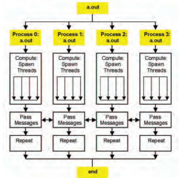
Figure 1. Four processes spawning four threads each
